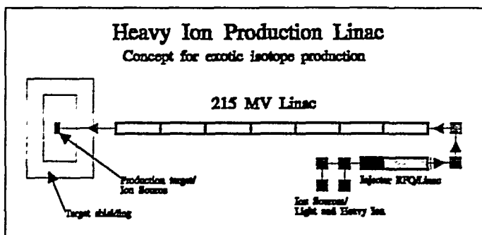
Fig. 1. Schematic view of a high beam power linac designed to deliver a variety of ion beams for radionuclide
