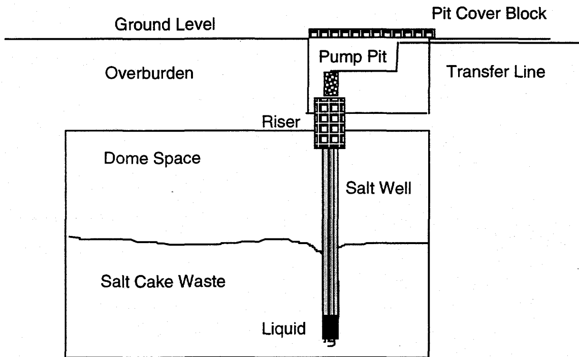
Fig. 1. Salt-Well Pumping
