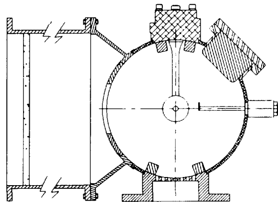
Fig. 3 Simplified DTL cross section.
