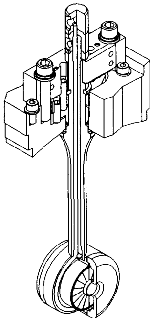
Fig. 2 Drift tube and mounting.
