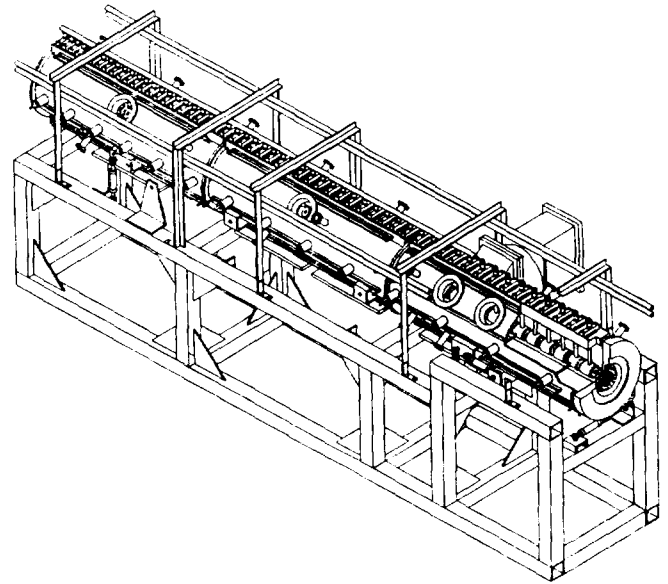
Fig. 1 Tank 1 on its frame.
