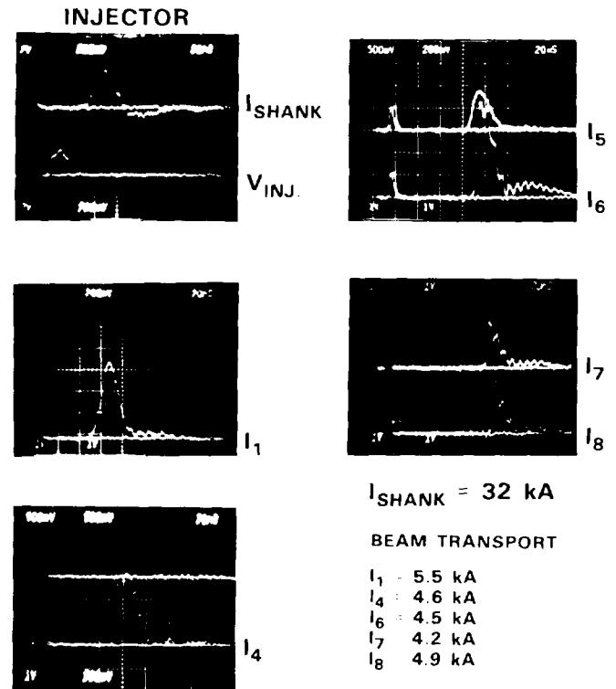
Fig. 2 Samples of the current wave forms. Only the injector was pulsed.
