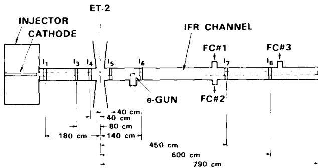
Fig. 1 Experimental set-up. Low energy 1.3MV injector.
