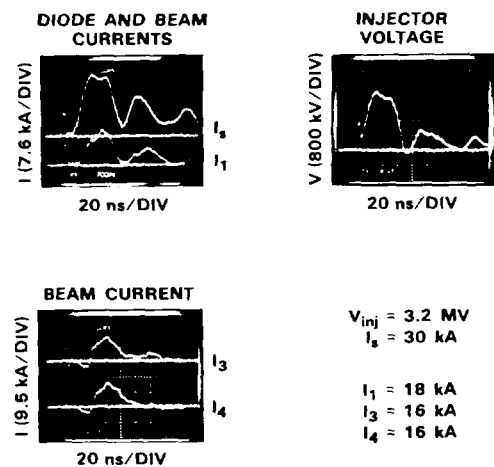
Fig. 6 Injector and beam current traces for a typical shot.
