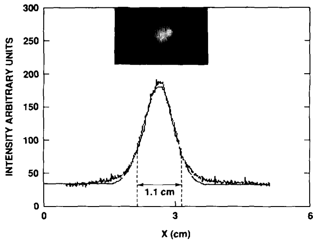
Fig. 7 Beam profile 440 cm downstream from the injector.
