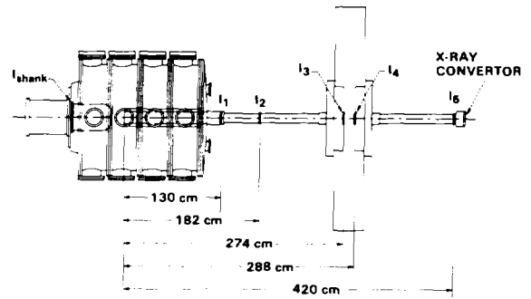
Fig. 4 Experimental set-up with the 4-MV injector. A re-entrant geometry is selected for the injector.
