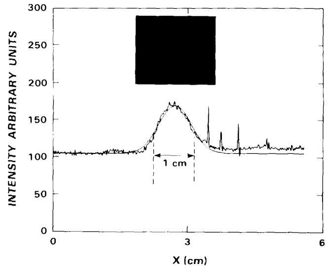
Fig. 5 Beam profile 130 cm downstream from injector diode.
