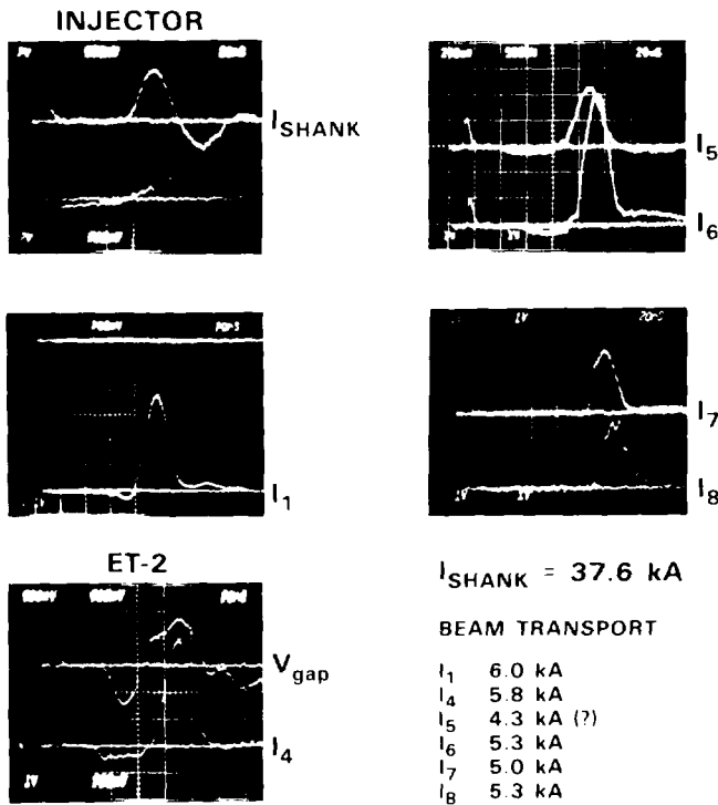
Fig. 3 Current wave forms with injector and ET-2 cavity pulsed in synchronism.
