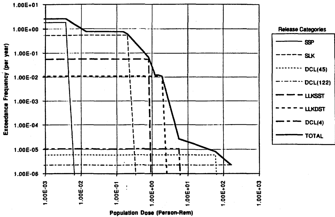
Fig. 8. Liquid total mean unconditional consequences.
