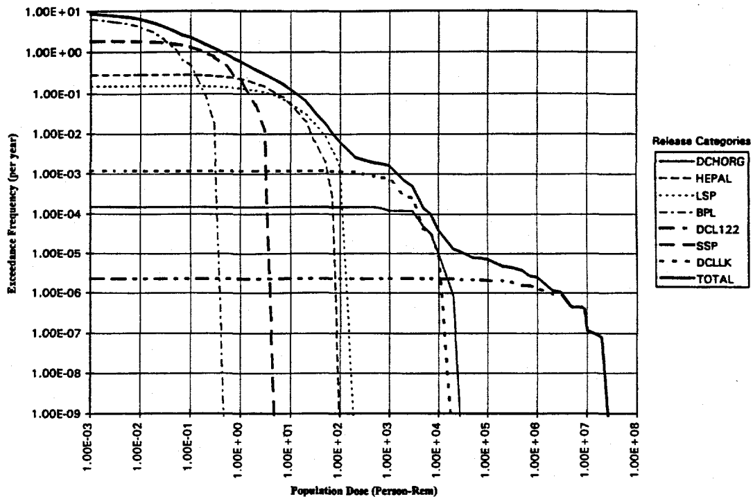
Fig. 4. Offsite total mean unconditional consequences.
