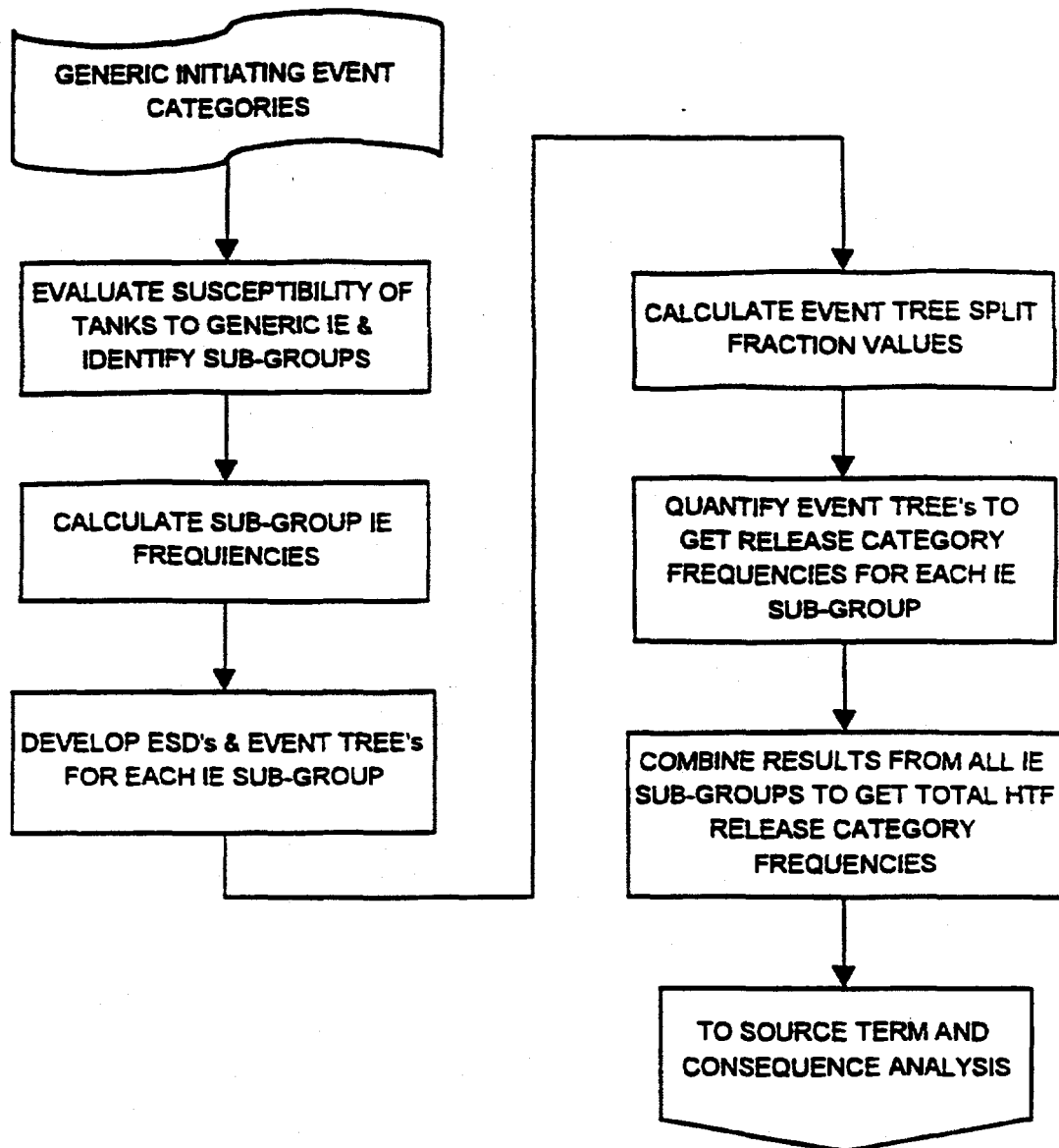
Fig. 2. Accident-sequence modeling steps.
