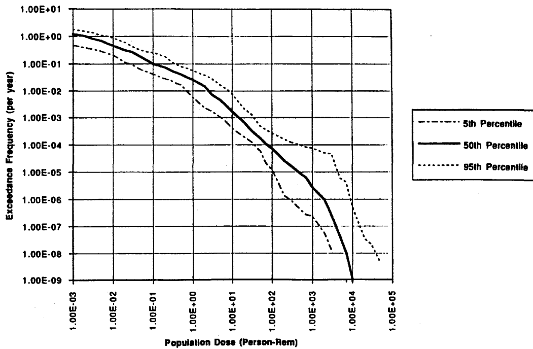
Fig. 7. Onsite total unconditional consequences.
