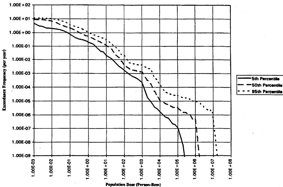
Fig. 5. Offsite total unconditional consequences.
