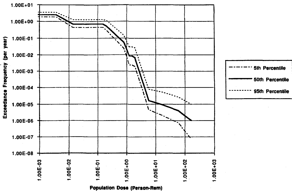
Fig. 9. Liquid total unconditional consequences.
