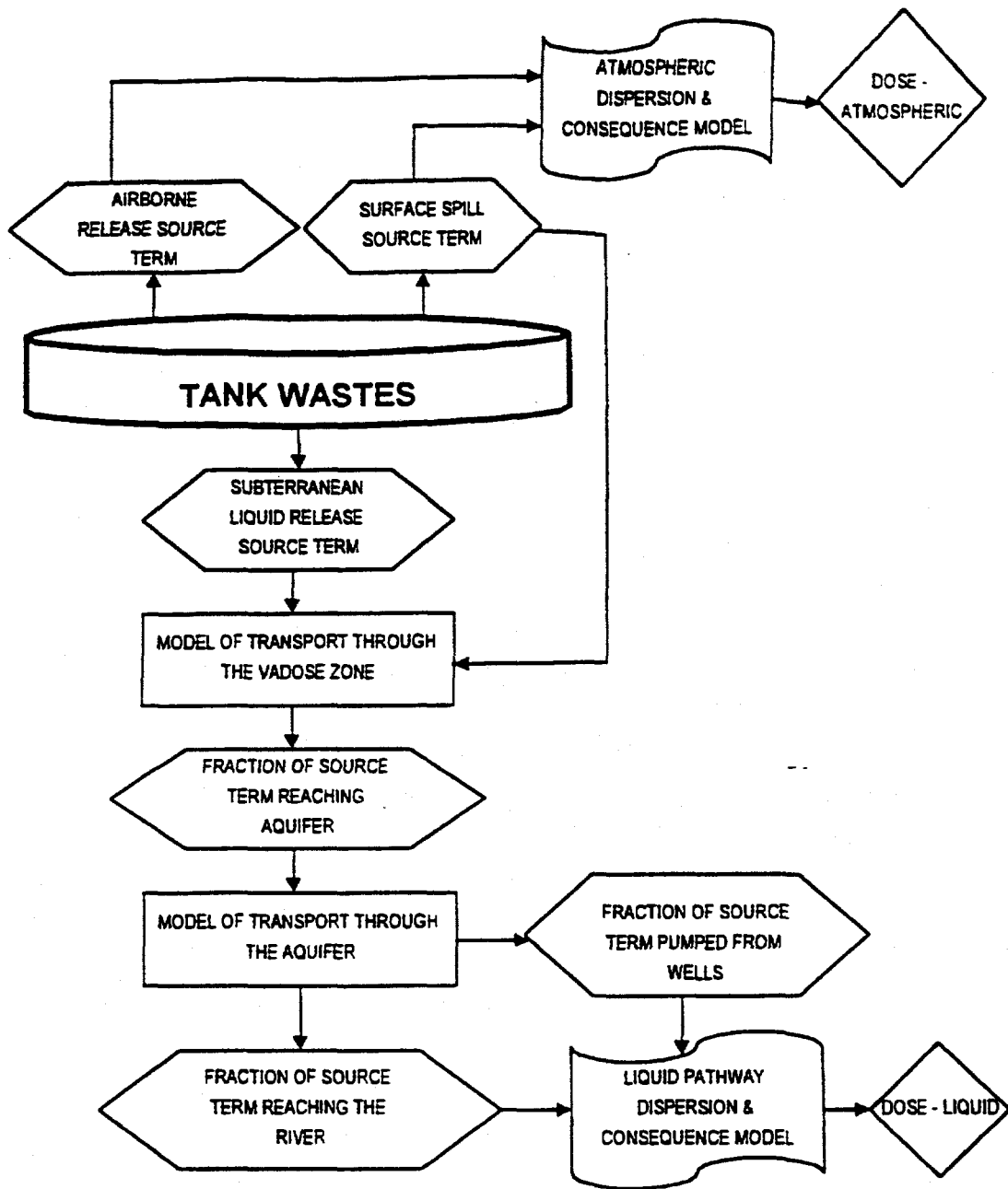
Fig. 3. HTF source term and consequence model assessment.
