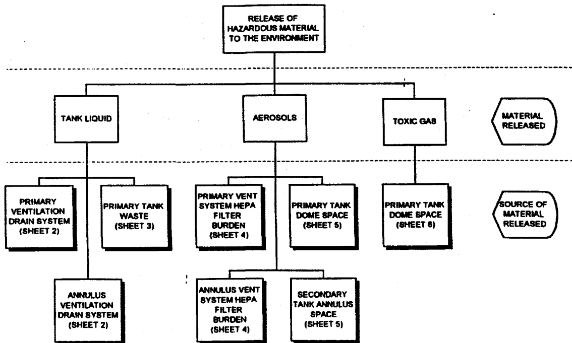
Fig. 1. Hanford Tank Farm Master Logic Diagram.
