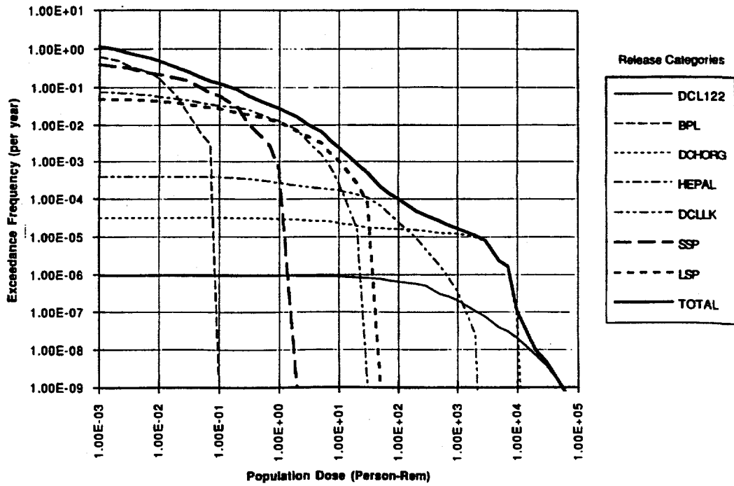
Fig. 6. Onsite total mean unconditional consequences.
