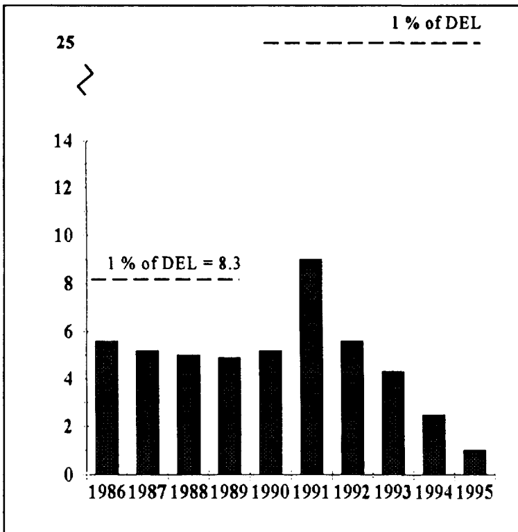
FIGURE 2.3 Noble Gas Effluent, Bruce "A", 1986-95 (TBq-MeV × 10 2 )
