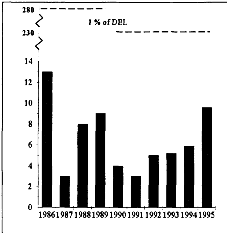
FIGURE 3.6 Gross Beta-Gamma Activity in Liquid Effluent, Bruce "B", 1986-95 (TBq × 10 -3 )
