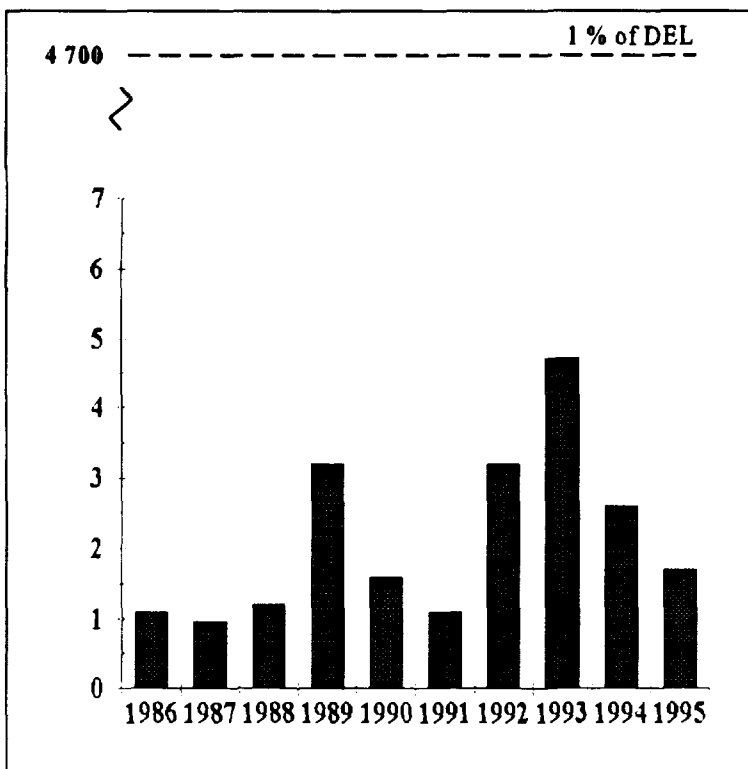
FIGURE 1.5 Tritium Oxide Liquid Effluent, Point Lepreau, 1986-95 (TBq × 10 2 )
