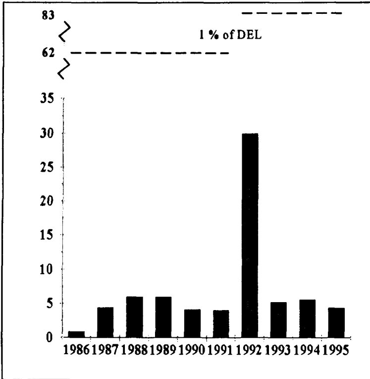
FIGURE 5.6 Tritium Oxide Liquid Effluent, Pickering "A", 1986-95 (TBq × 10 2 )
