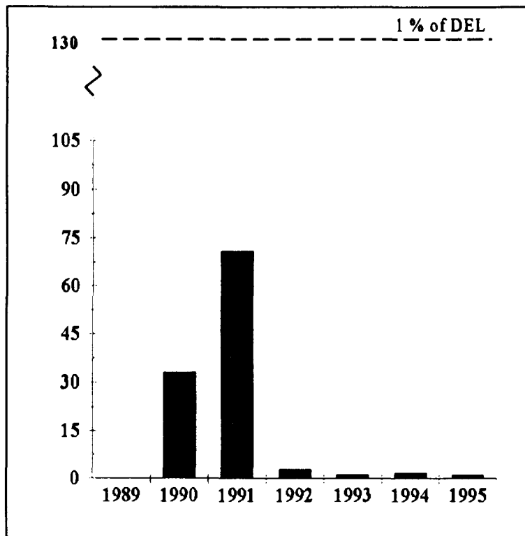
FIGURE 4.6 Gross Beta-Gamma Activity in Liquid Effluent, Darlington, 1989-95 (TBq × 10 -2 )
