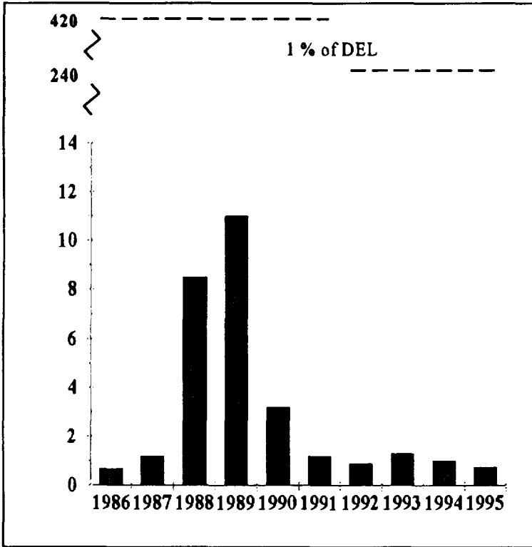
FIGURE 5.2 Iodine-131 Gaseous Effluent, Pickering "A", 1986-95 (TBq × 10 -4 )
