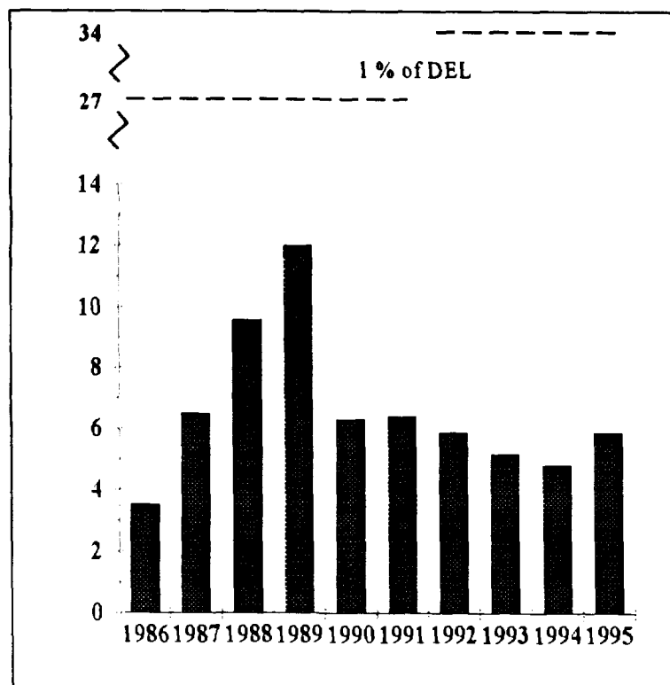
FIGURE 5.1 Tritium Oxide Gaseous Effluent, Pickering "A", 1986-95 (TBq × 10 2 )
