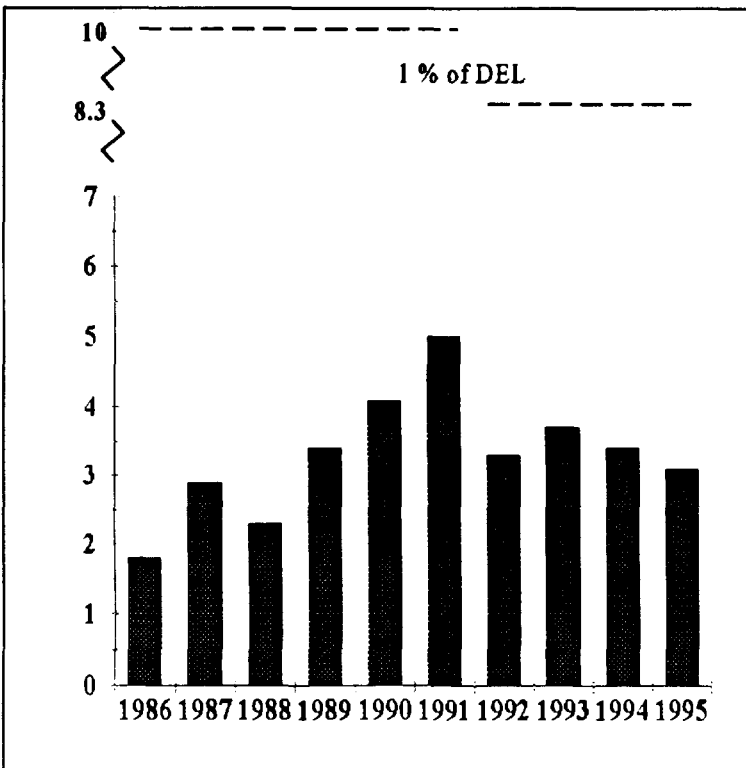
FIGURE 5.3 Noble Gas Effluent, Pickering "A", 1986-95 (TBq-MeV × 10 2 )
