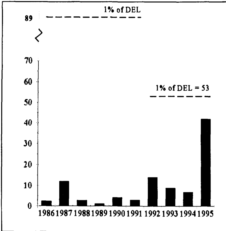
FIGURE 7.6 Gross Beta-Gamma Activity in Liquid Effluent, Gentilly-2, 1986-95 (TBq × 10 -3 )
