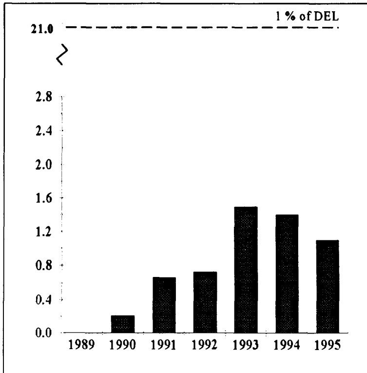
FIGURE 4.3 Noble Gas Effluent, Darlington, 1989-95 (TBq-MeV × 10 2 )
