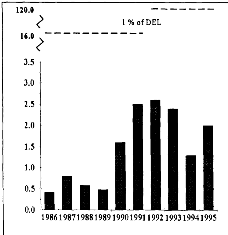
FIGURE 7.5 Tritium Oxide Liquid Effluent, Gentilly-2, 1986-95 (TBq × 10 2 )
