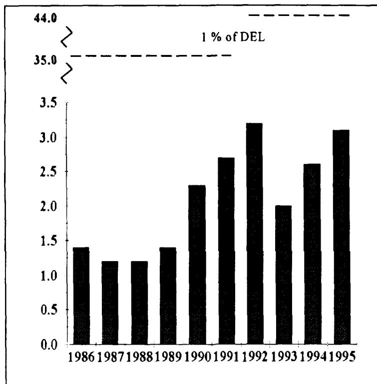
FIGURE 7.1 Tritium Oxide Gaseous Effluent, Gentilly-2, 1986-95 (TBq × 10 2 )
