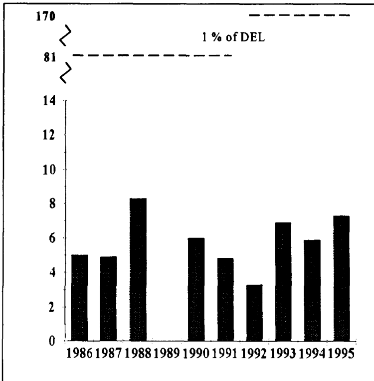
FIGURE 7.3 Noble Gas Effluent, Gentilly-2, 1986-95 (TBq-MeV × 10 1 )
