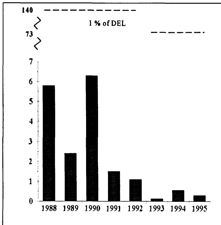
FIGURE 4.7 Elemental Tritium Gaseous Effluent, Darlington, 1988-95 (TBq × 10 3 )
