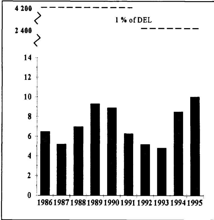
FIGURE 6.2 Iodine-131 Gaseous Effluent, Pickering "B", 1986-95 (TBq × 10 -5 )
