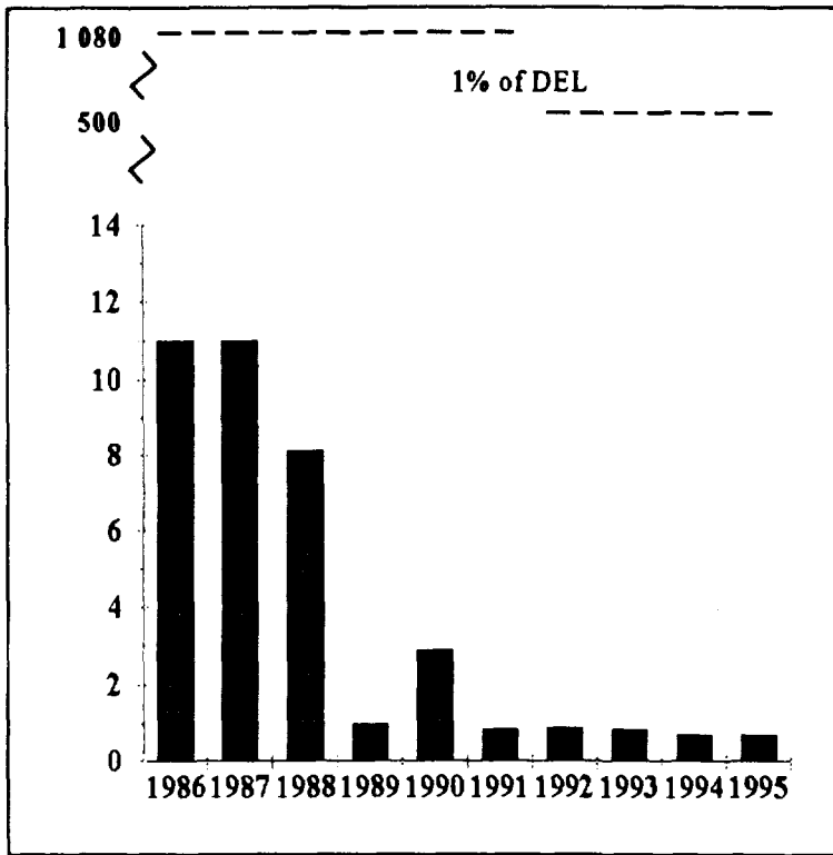
FIGURE 5.4 Radioactive Particulates in Gaseous Effluent, Pickering "A", 1986-95 (TBq × 10 -4 )
