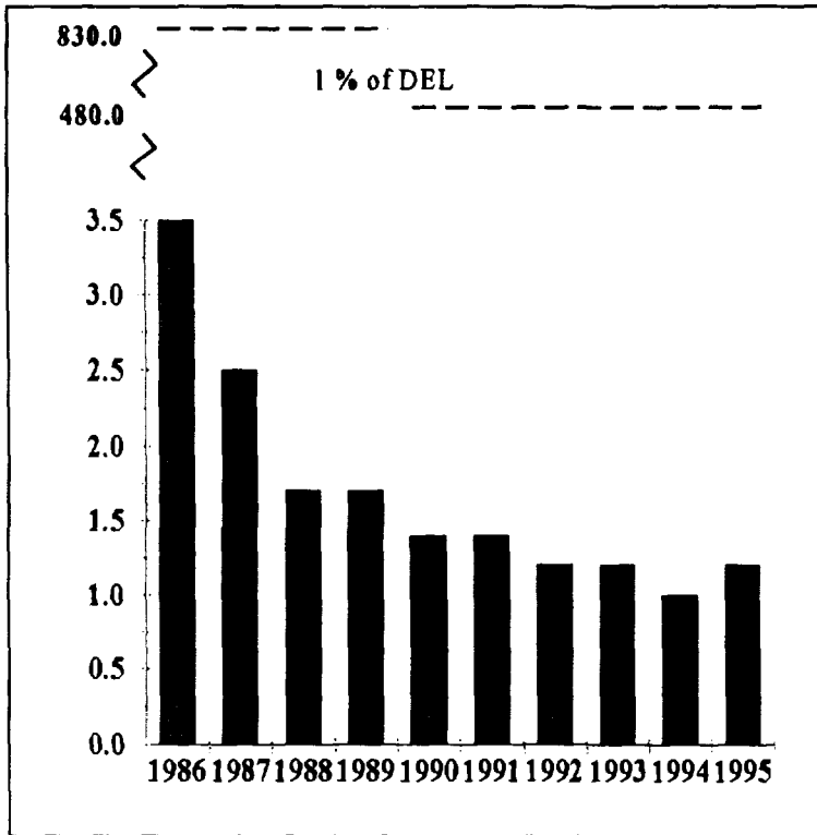
FIGURE 3.4 Radioactive Particulates in Gaseous Effluent, Bruce "B", 1986-95 (TBq × 10 -4 )
