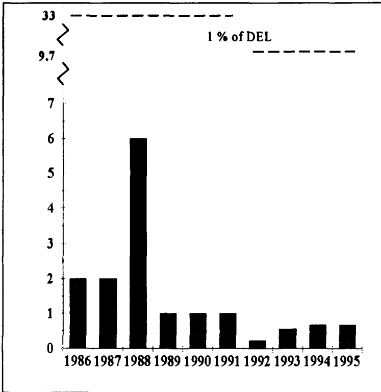
FIGURE 6.6 Gross Beta-Gamma Activity in Liquid Effluent, Pickering "B", 1986-95 (TBq × 10 -2 )
