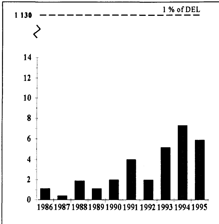
FIGURE 1.6 Gross Beta-Gamma Activity in Liquid Effluent, Point Lepreau, 1986-95 (TBq × 10 -3 )
