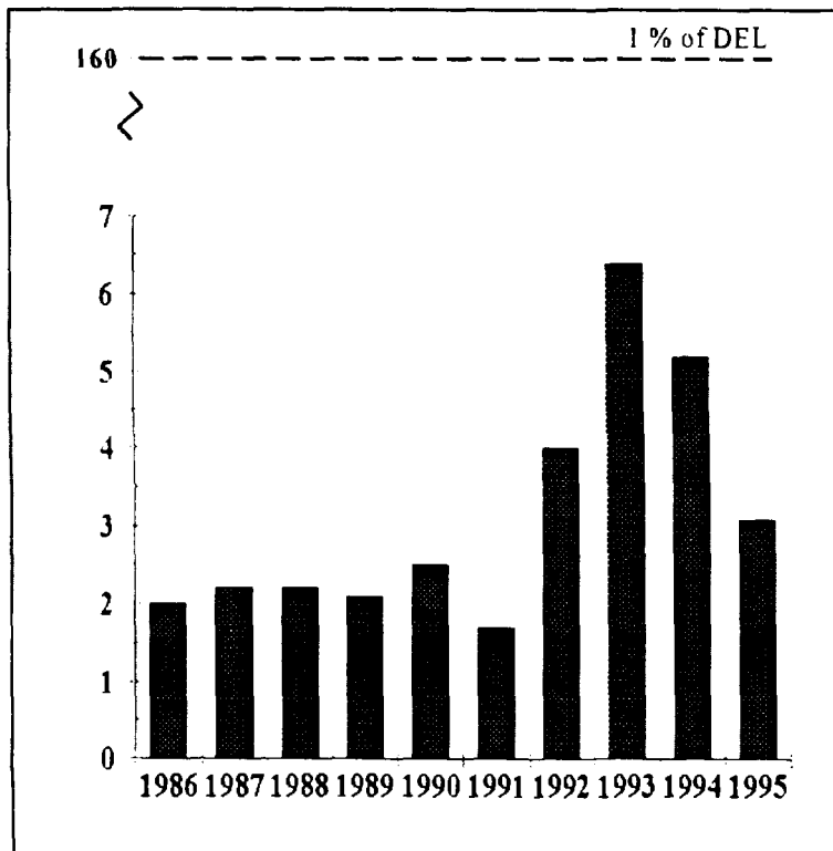
FIGURE 1.1 Tritium Oxide Gaseous Effluent, Point Lepreau, 1986-95 (TBq × 10 2 )
