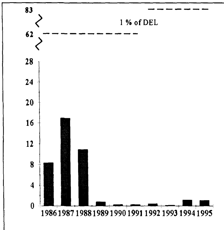
FIGURE 6.5 Tritium Oxide Liquid Effluent, Pickering "B", 1986-95 (TBq × 10 2 )
