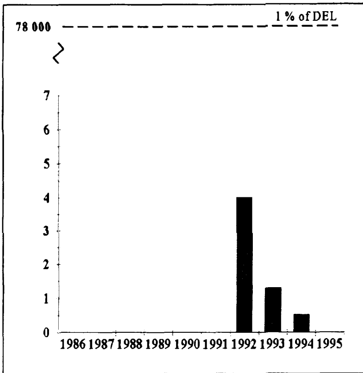
FIGURE 1.4 Radioactive Particulates in Gaseous Effluent, Point Lepreau, 1986-95 (TBq × 10 -6 )
