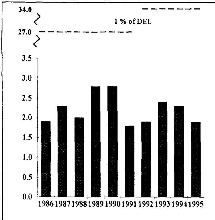
FIGURE 6.1 Tritium Oxide Gaseous Effluent, Pickering "B", 1986-95 (TBq × 10 2 )
