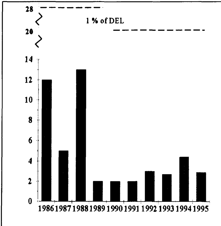
FIGURE 2.6 Gross Beta-Gamma Activity in Liquid Effluent, Bruce "A", 1986-95 (TBq × 10 -2 )
