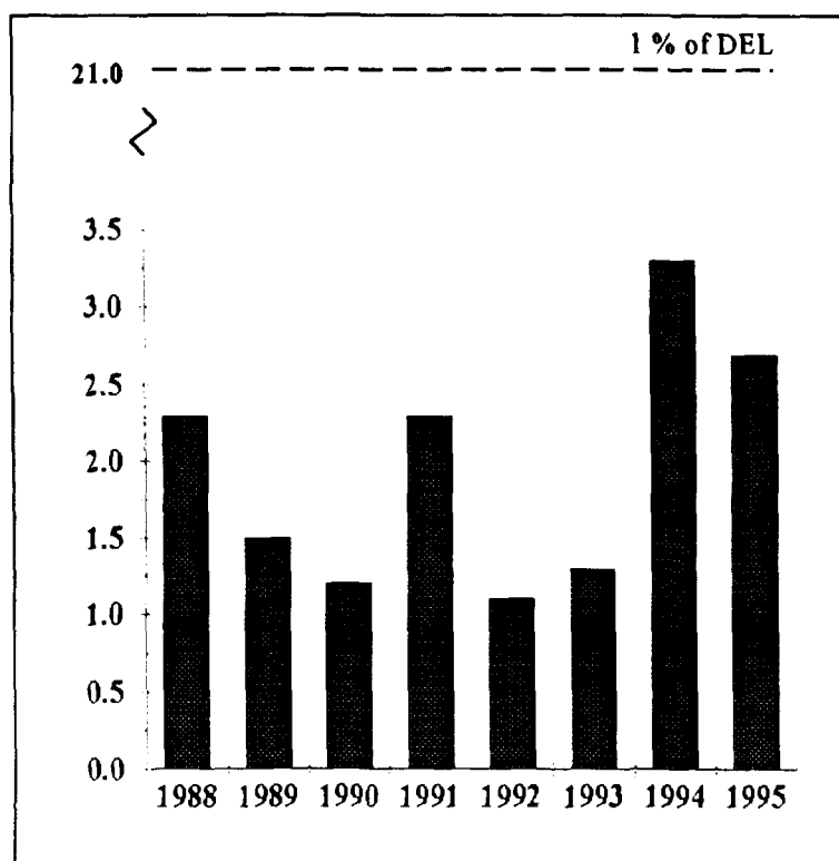
FIGURE 4.1 Tritium Oxide Gaseous Effluent, Darlington, 1988-95 (TBq × 10 2 )
