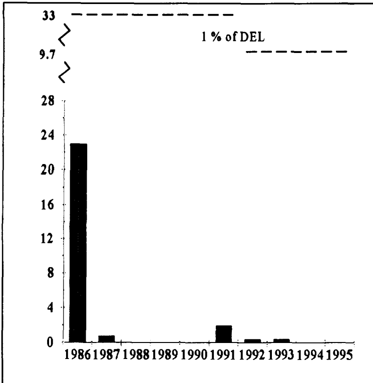
FIGURE 7.2 Iodine-131 Gaseous Effluent, Gentilly-2, 1986-95 (TBq × 10 -5 )
