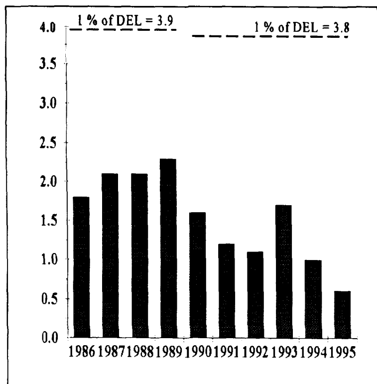
FIGURE 2.1 Tritium Oxide Gaseous Effluent, Bruce "A", 1986-95 (TBq \times 10^3 )
