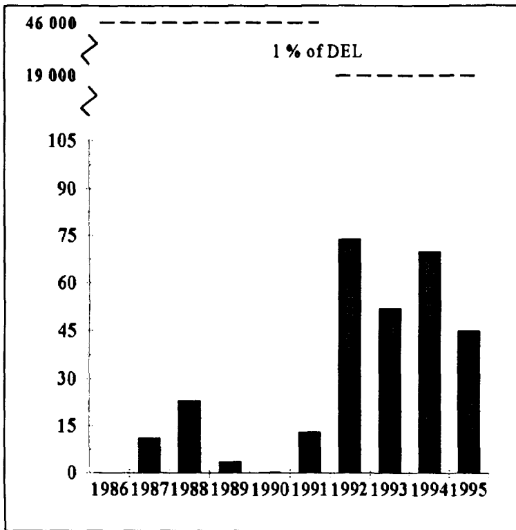
FIGURE 7.4 Radioactive Particulates in Gaseous Effluent, Gentilly-2, 1986-95 (TBq × 10 -6 )
