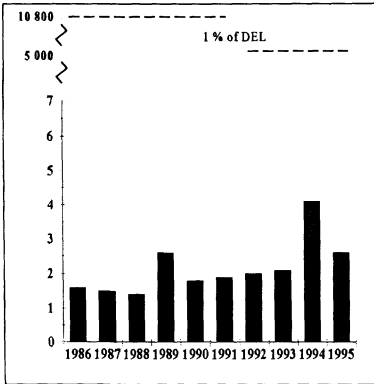
FIGURE 6.4 Radioactive Particulates in Gaseous Effluent, Pickering "B", 1986-95 (TBq × 10 -5 )
