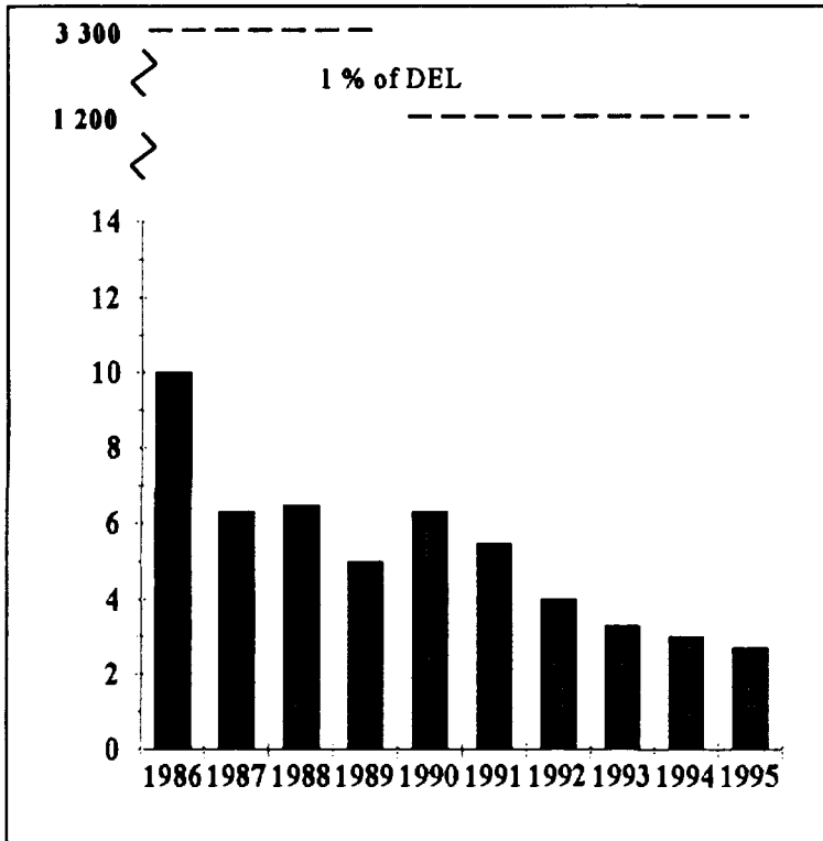
FIGURE 2.2 Iodine-131 Gaseous Effluent, Bruce "A", 1986-95 (TBq × 10 -5 )
