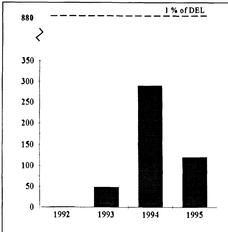
FIGURE 7.7 Carbon-14 in Gaseous Effluent, Gentilly-2, 1992-95 (TBq × 10 -2 )
