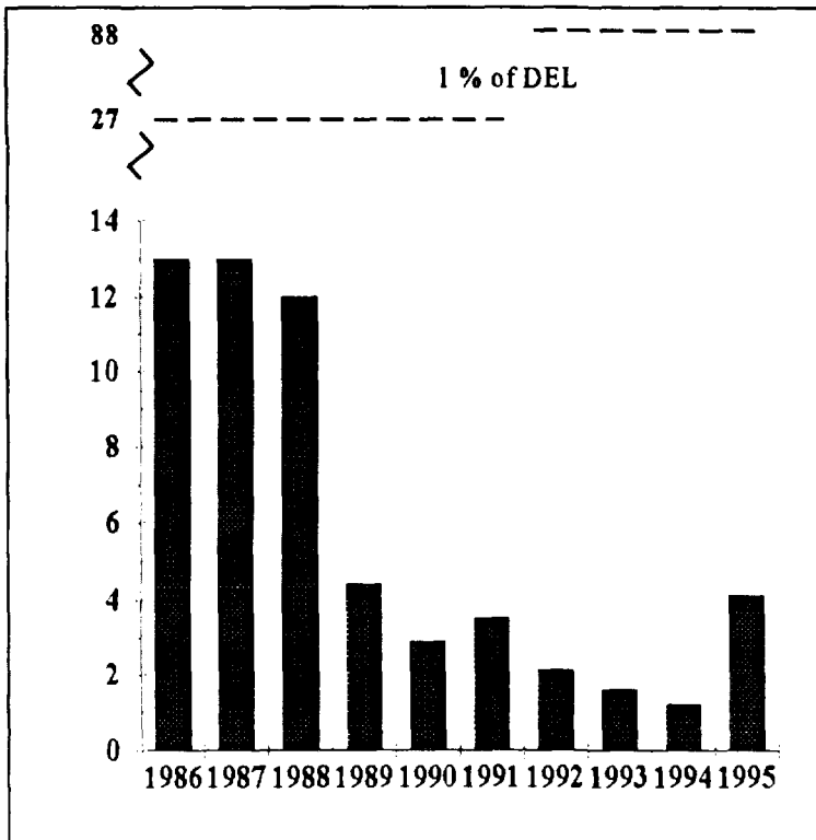
FIGURE 5.5 Carbon-14 in Gaseous Effluent, Pickering "A", 1986-95 (TBq)
