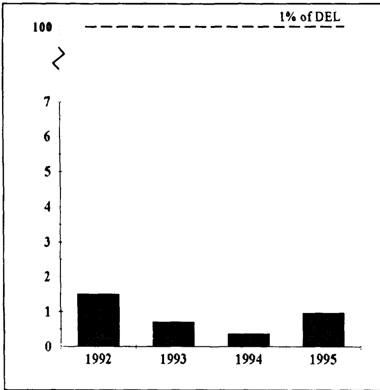
FIGURE 7.8 Carbon-14 in Liquid Effluent, Gentilly-2, 1992-95 (TBq × 10 -2 )
