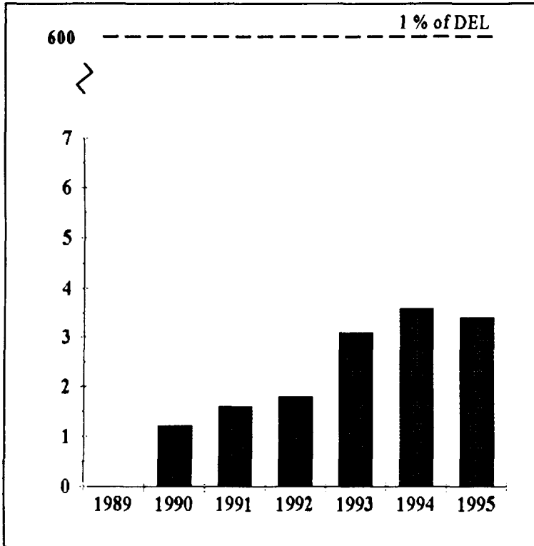
FIGURE 4.2 Iodine-131 Gaseous Effluent, Darlington, 1989-95 (TBq × 10 -5 )
