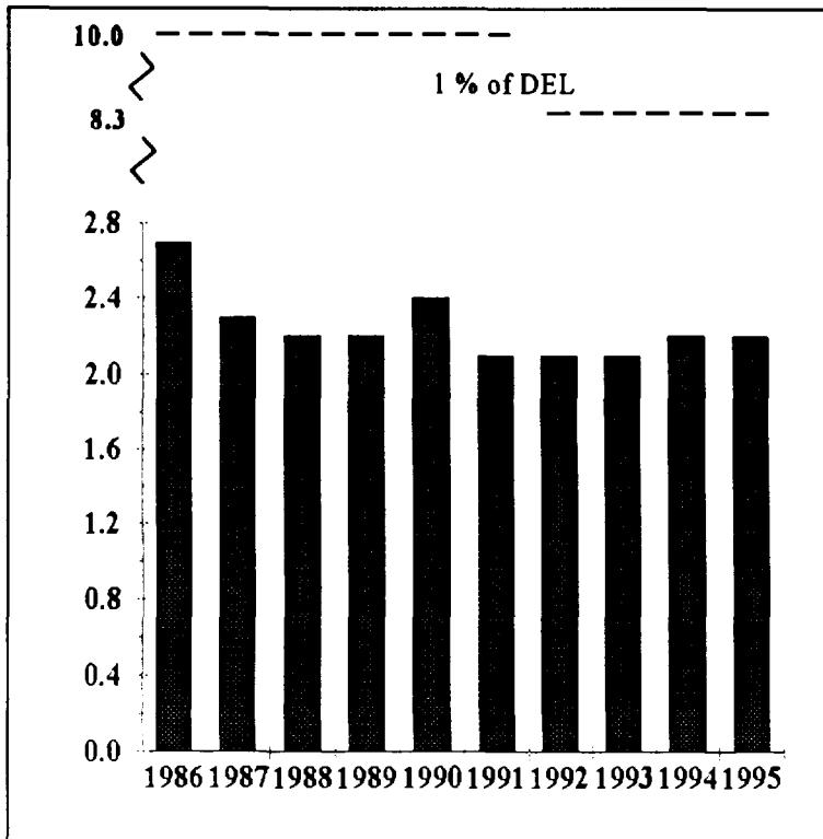
FIGURE 6.3 Noble Gas Effluent, Pickering "B", 1986-95 (TBq-MeV × 10 2 )
