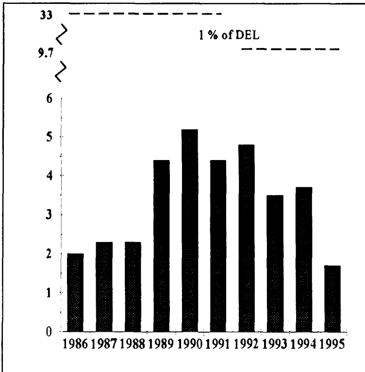
FIGURE 5.7 Gross Beta-Gamma Activity in Liquid Effluent, Pickering "A", 1986-95 (TBq × 10 -2 )
