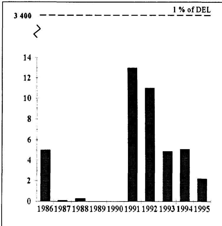
FIGURE 1.3 Noble Gas Effluent, Point Lepreau, 1986-95 (TBq-MeV)
