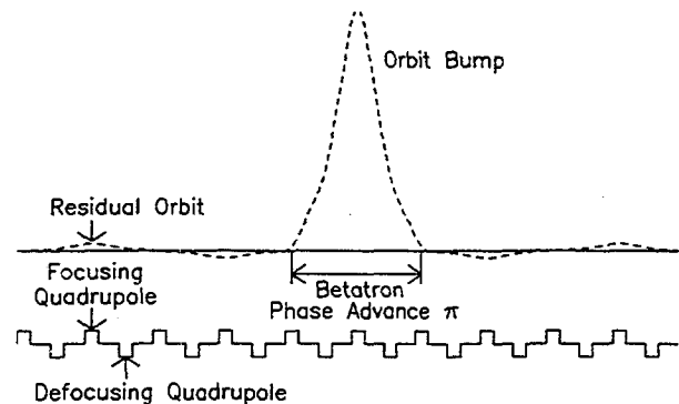
Figure 2. Measurement of quadrupole gradient error using an orbit bump with betatron phase advance of \pi .
