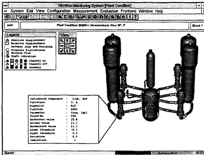
Figure 8 - SÜS '95 displays the location of an affected reactor coolant system component
