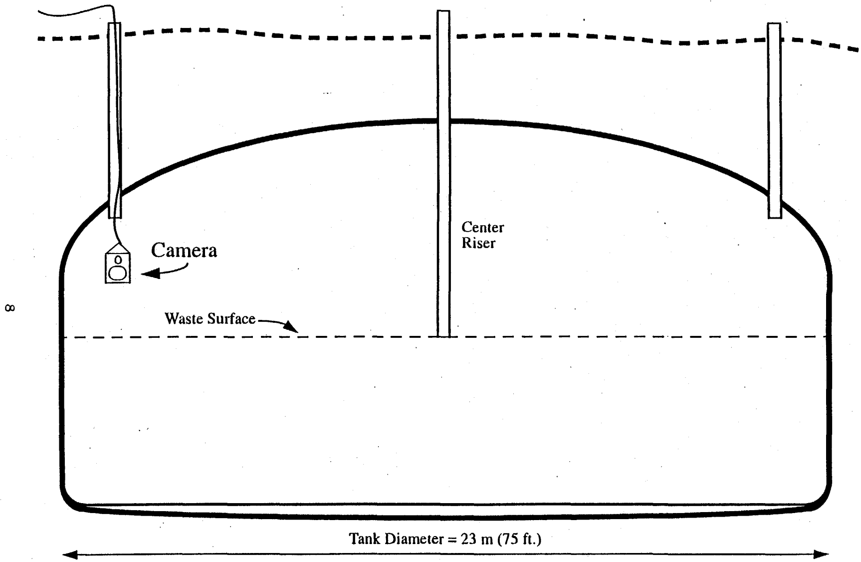
FIGURE 5 Single shell tank cross section.
