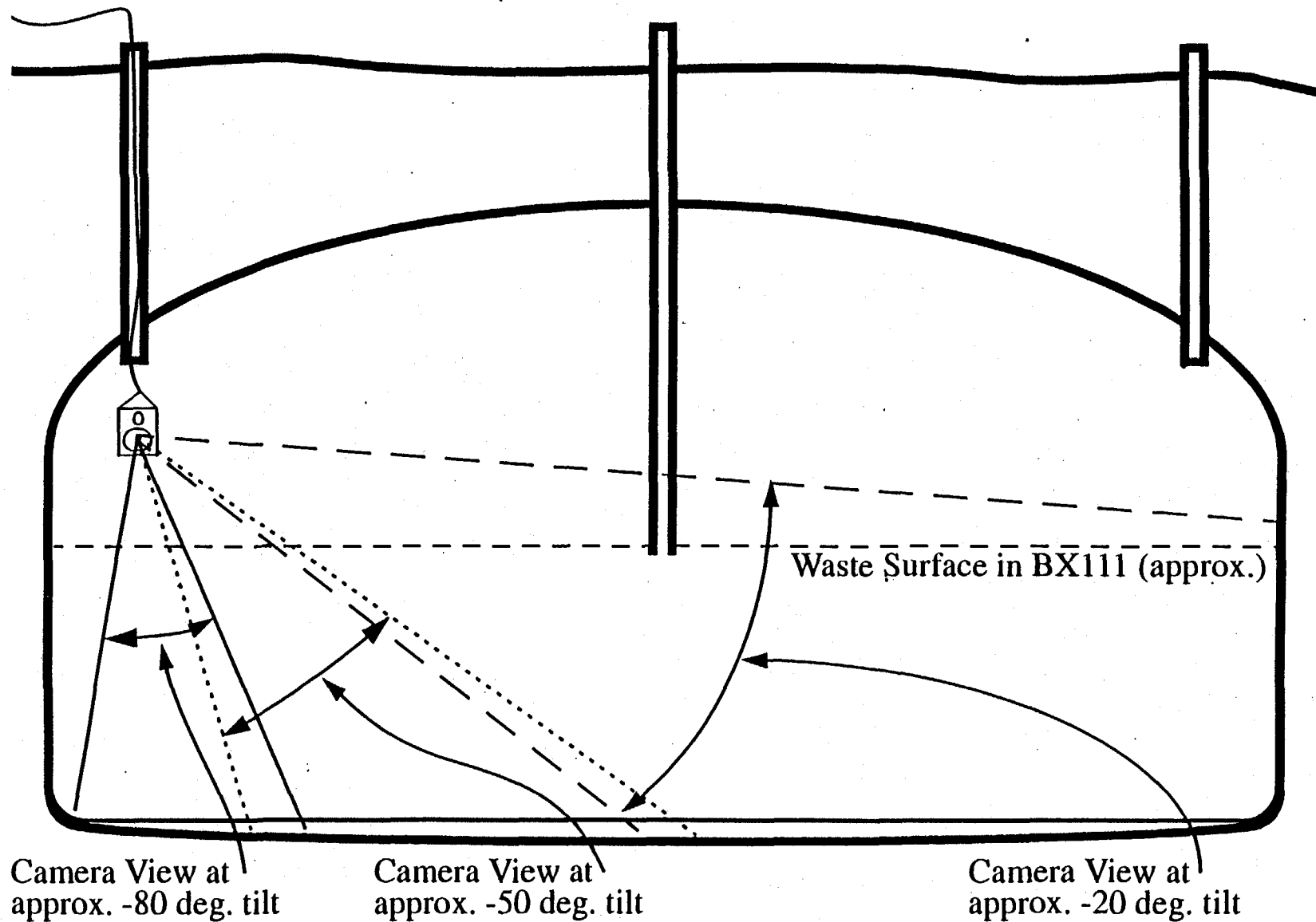
FIGURE 6 Camera positions and fields of view at approximately -20°, -50°, and -80°.
