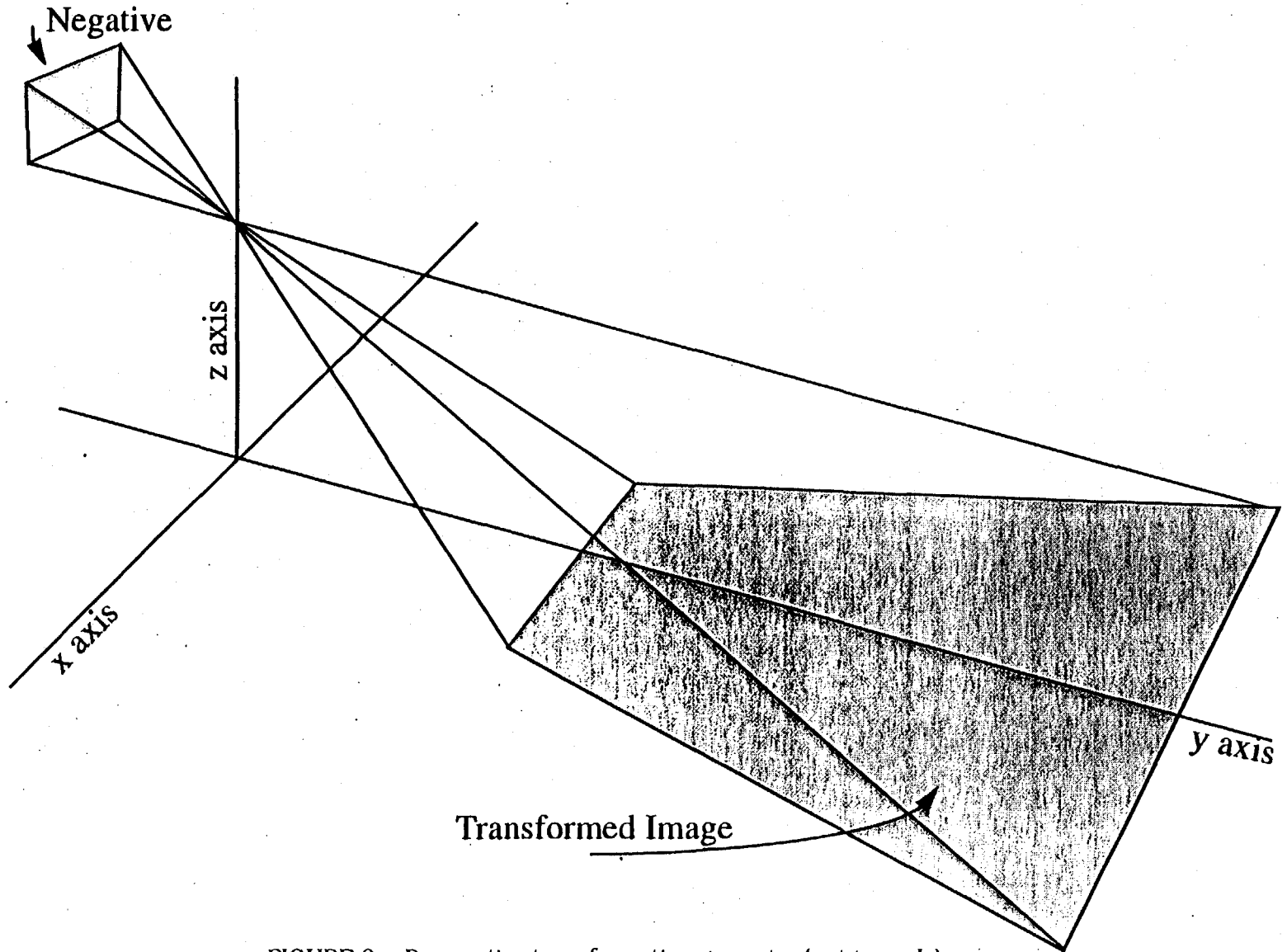
FIGURE 8 Perspective transformation geometry (not to scale).
