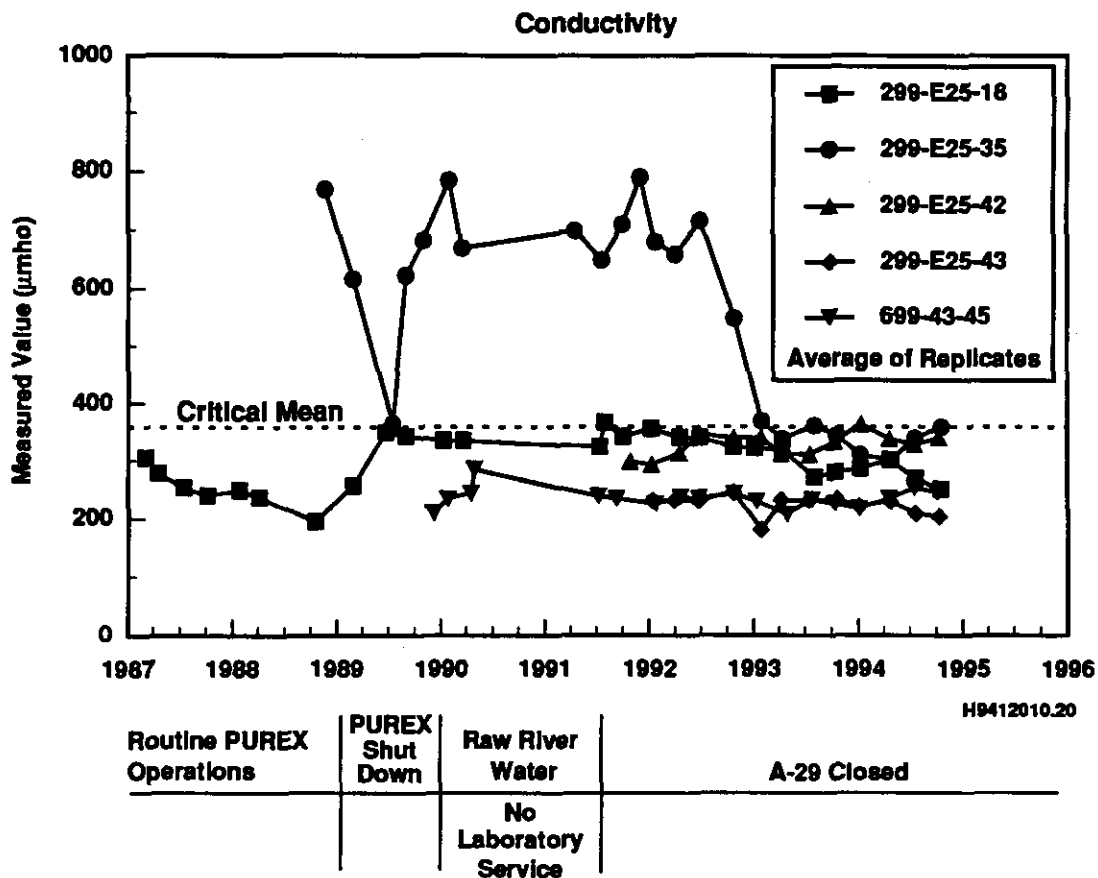
Figure 8. Specific Conductance and Sulfate Concentrations Over Time at Well 299-E25-35 and Select Wells.
