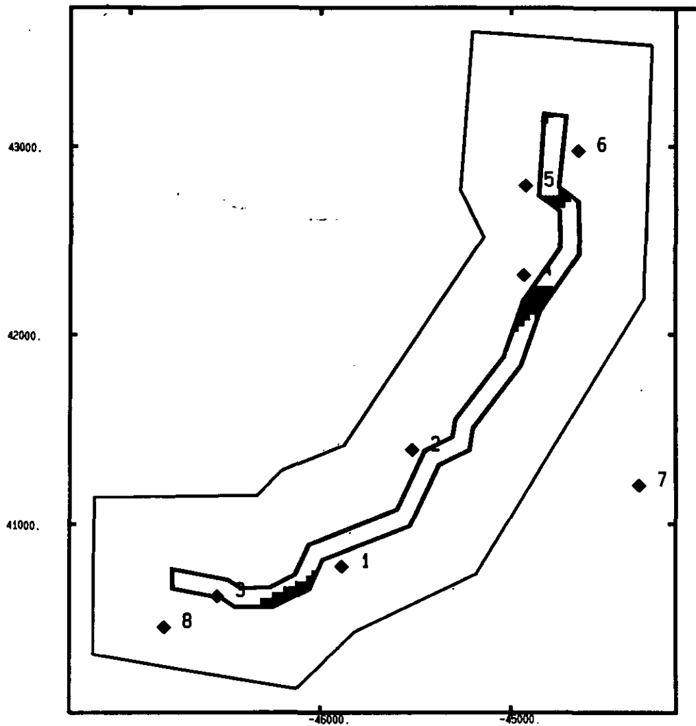
Figure 11. 216-A-29 Ditch MEMO Results.
