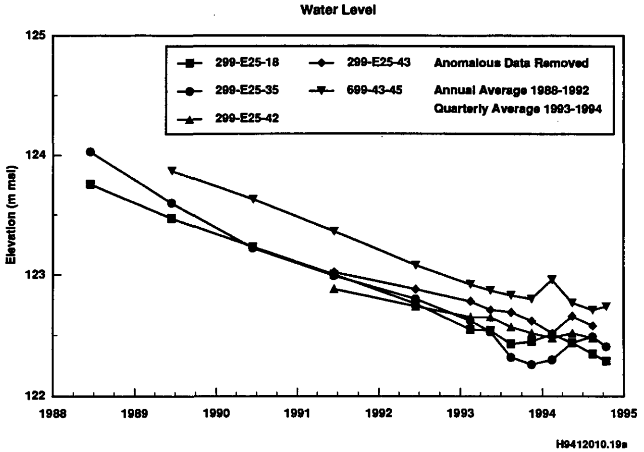
Figure 6. Hydrograph of Select 216-A-29 Ditch Monitoring Wells (Freeman 1994a).
