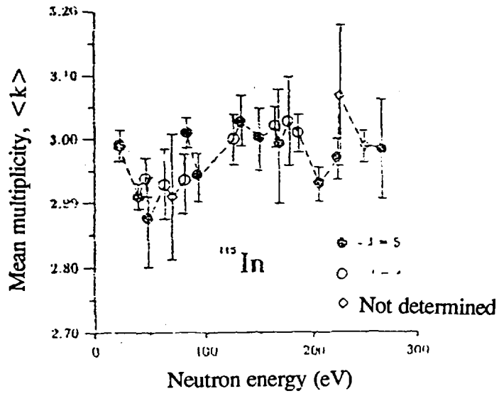
Fig. 3. Dependence of the mean multiplicity on resonance energy for indium-115.
