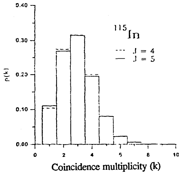
Fig. 4. Experimental distribution of the gamma ray multiplicity for resonances with different spins in indium-115.
