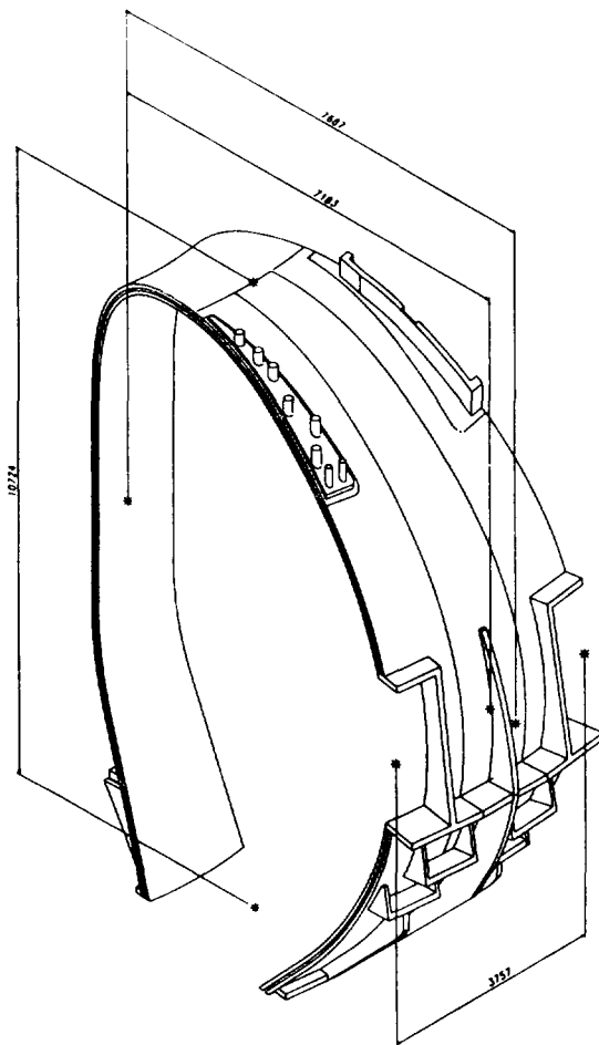
Figure 8. Backplate Sector
