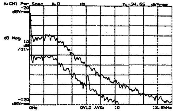
Fig. 4. BPM output noise spectrum with no input signal (upper trace) and with input power = 0 \text{ dBm} (lower trace).
