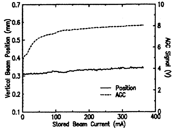
Fig. 5. BPM vertical output signal and AGC voltage during injection into the X-ray storage ring.
