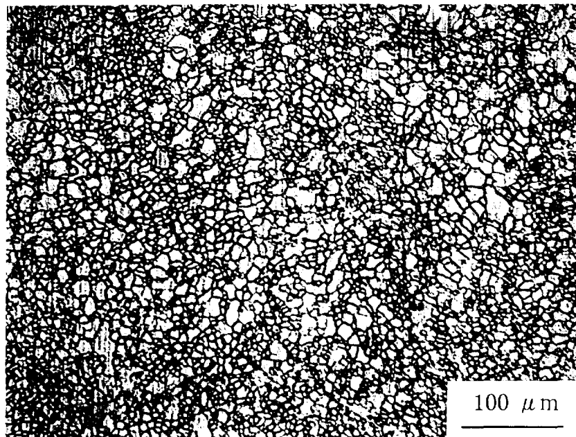
Fig. 10. Optical micrograph of recrystallized structure of technetium metal.
