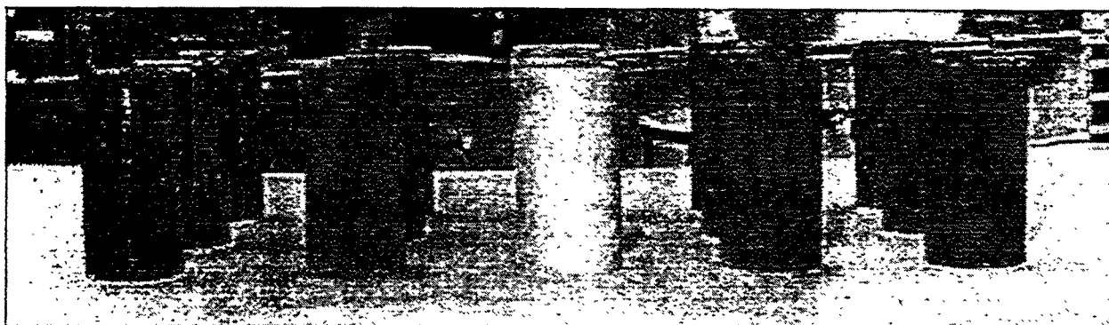
Figure 3. Stabilized Soil Samples from the INEEL Acid Pit Treatability Study.
