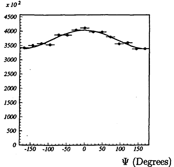
Figure 6. Distribution of relative angles \Psi between proton and light-particle ( A > 1 ) flow directions measured in the target rapidity region with the Plastic Ball of WA98 for intermediate centrality 158 A GeV Pb + Pb collisions.
