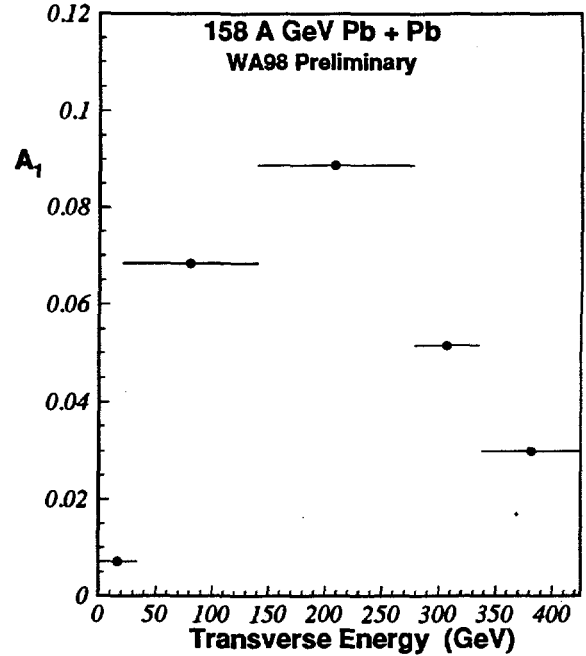
Figure 7. Strength of correlation between proton and light particle ( A > 1 ) flow directions as a function of centrality in 158 A GeV Pb + Pb collisions.
