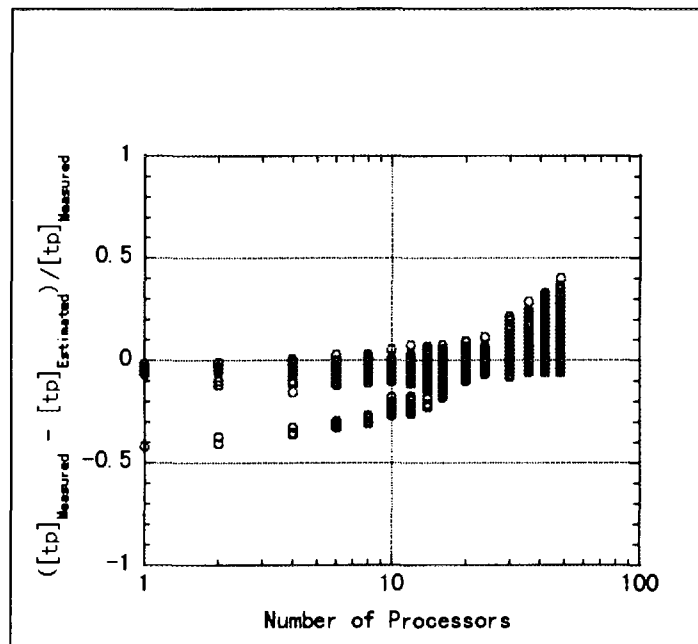
Fig.18b Accuracy of timing model of do302 of propcel with p.
