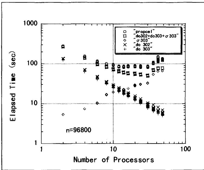
Fig. 9b Processing time of prope1, do302, do303 and σ 303.
