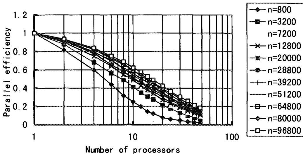
Fig.6 SP2 parallel performance with parallel efficiency.
