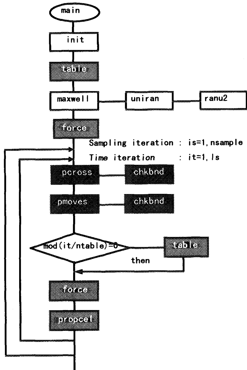
Fig.2 Flowchart of molecular dynamics(MD) code.
