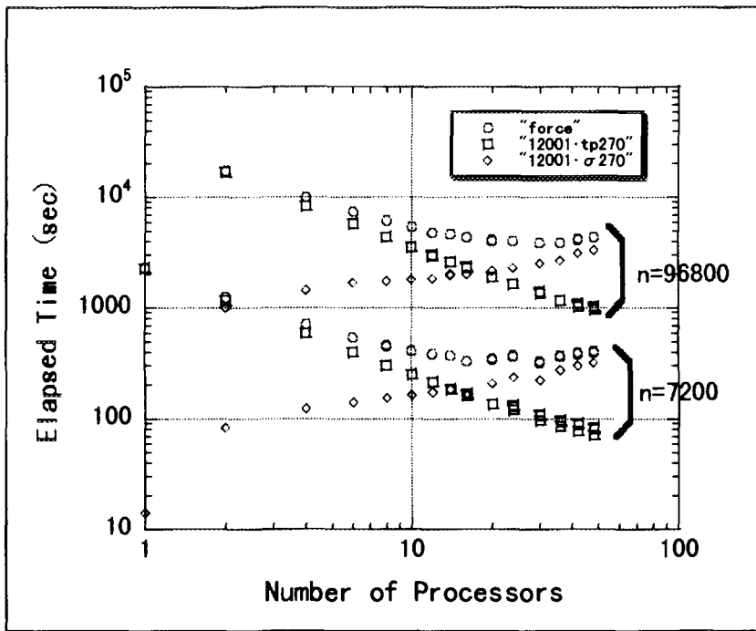
Fig. 9a Processing time of force, do270 and σ 270.
