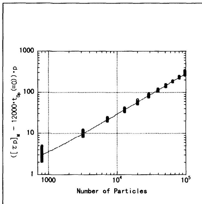
Fig.17 Least square fitting of [\tau_p(p, n)]_M - 12000 \cdot t_{0p302} vs. n .
