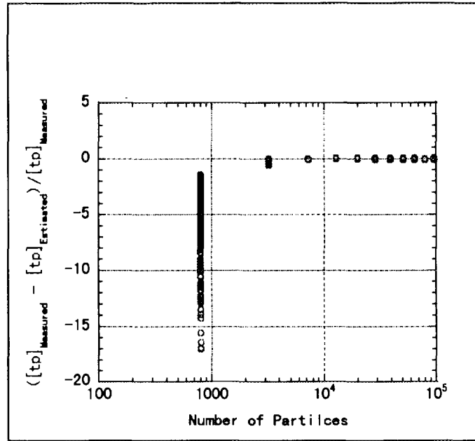
Fig.16a Accuracy of timing model of table with n.
