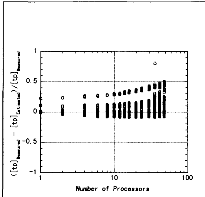
Fig.20b Accuracy of timing model of do303 of propcel with p.
