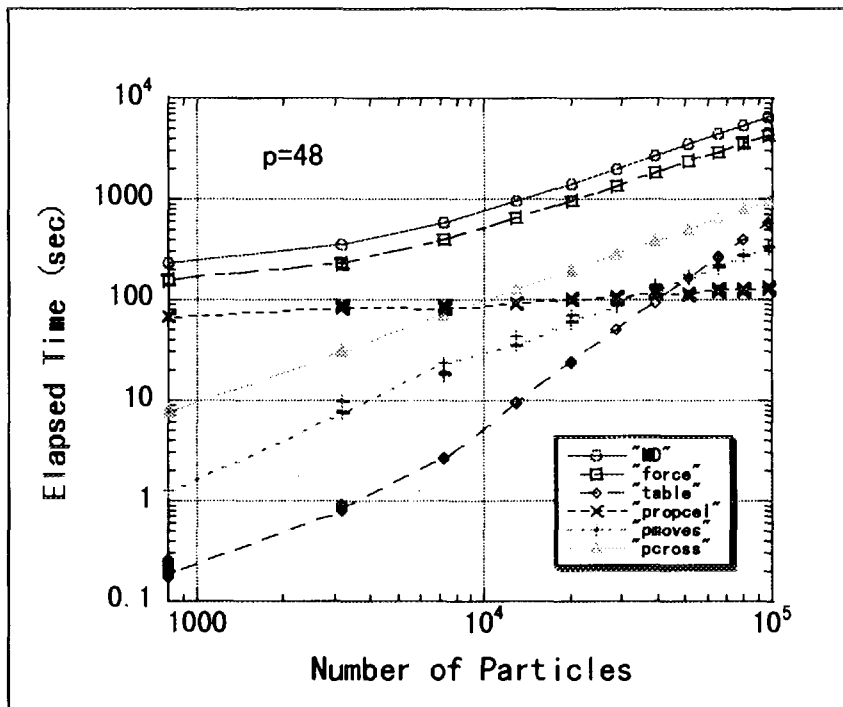
Fig. 7b Processing time(p=48) of MD code and subroutines.
