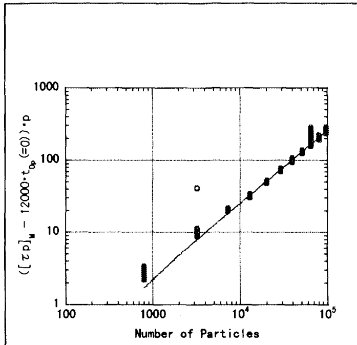
Fig.19 Least square fitting of [\tau_p(p,n)]_M - 12000 \cdot t_{0p303} vs. n . (3) t_{0n303} , a_{u303}
