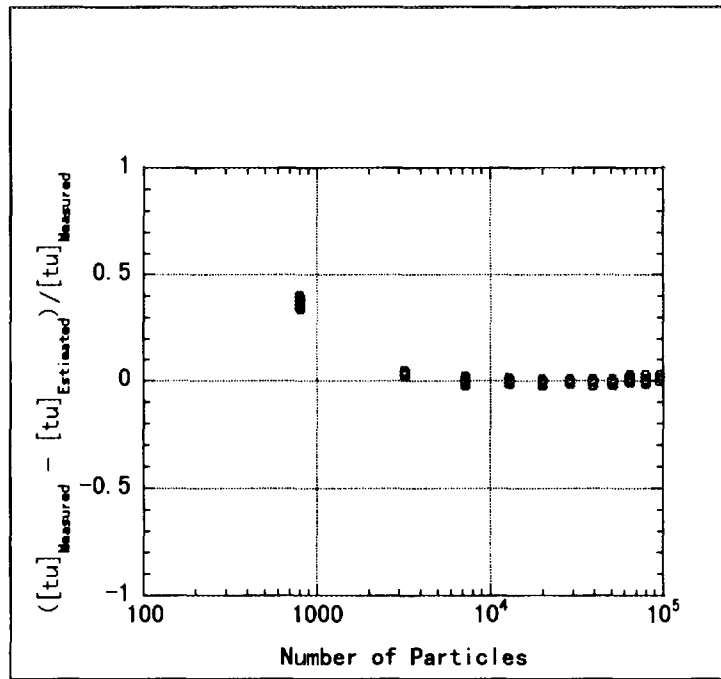
Fig.23 Accuracy of timing of pcross with n.
