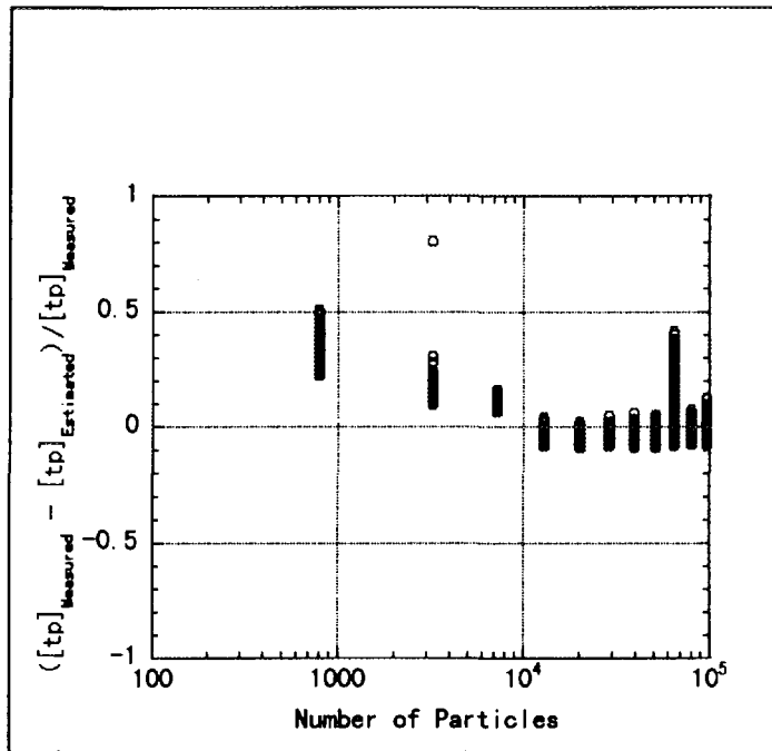
Fig.20a Accuracy of timing model of do303 of propcel with n.
