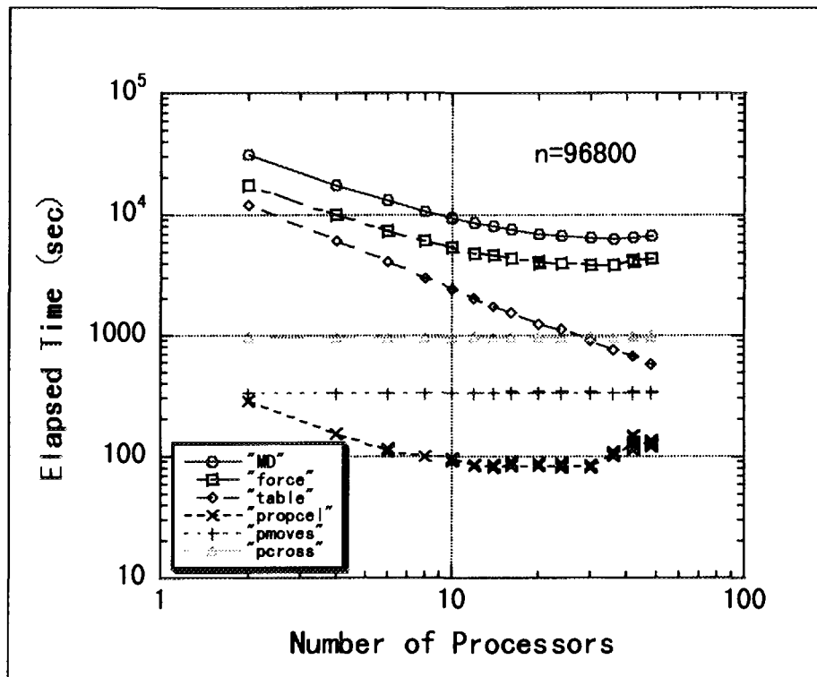
Fig. 8b Processing time( n=96800 ) of MD code and subroutines.
