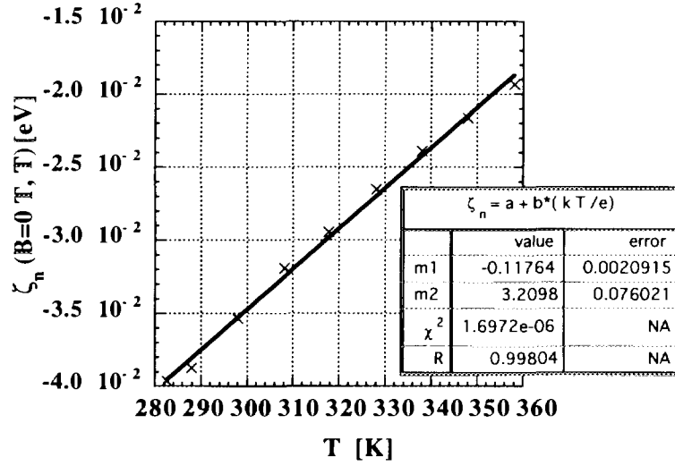
FIG. 10. Temperature dependence of the Fermi level. The experimental results are fitted by \zeta_n = -0.117 + 3.2 \frac{kT}{|e|} [ eV ]. This equation denotes that E_G \approx 0.23 [ eV ] and m_p/m_n \approx 73 .
