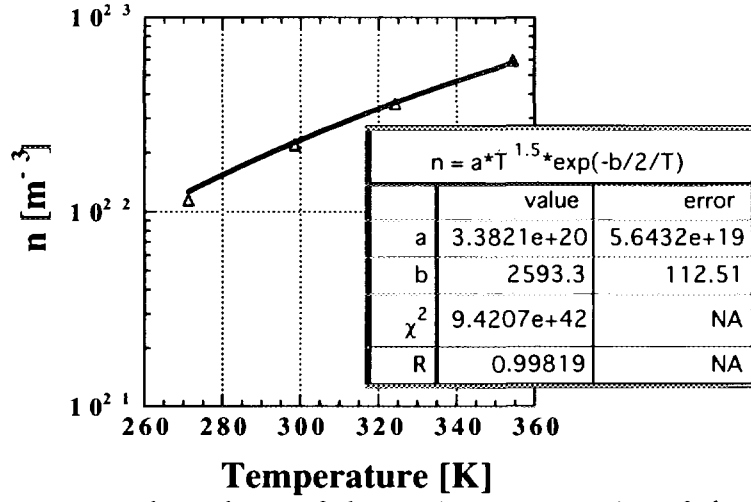
FIG. 7. Temperature dependence of the carrier concentration of the electron. Fitting function is n(T) = 3.3 \times 10^{20} T^{1.5} \exp\left(-\frac{2600}{kT}\right) . Comparing the intrinsic concentration eq. (13), we have E_G \approx 0.22 [eV] and m_n m_p \approx 1.7 \times 10^{-2} m_0^2 .
