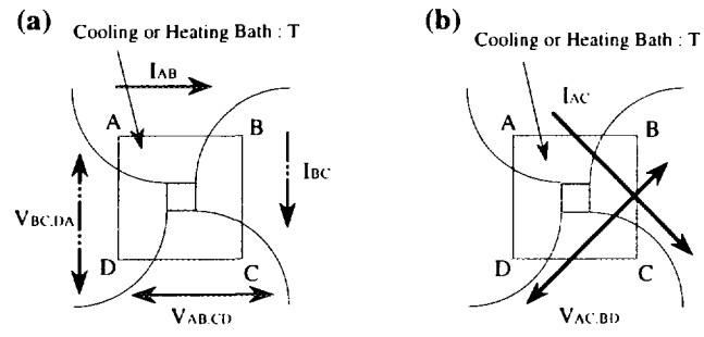
FIG. 2. Sample geometries for performing (a) resistivity and (b) Hall measurements by the van der Pauw method. Size of sample is 4\text{mm} \times 4\text{mm} \times 1\text{mm} .
