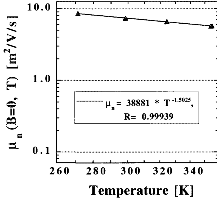
FIG. 8. Temperature dependence of the electron mobility. The experimental results are fitted by \mu_n \approx 7.5 \times (T/300)^{-1.50} [\text{m}^2/\text{V/s}] .
