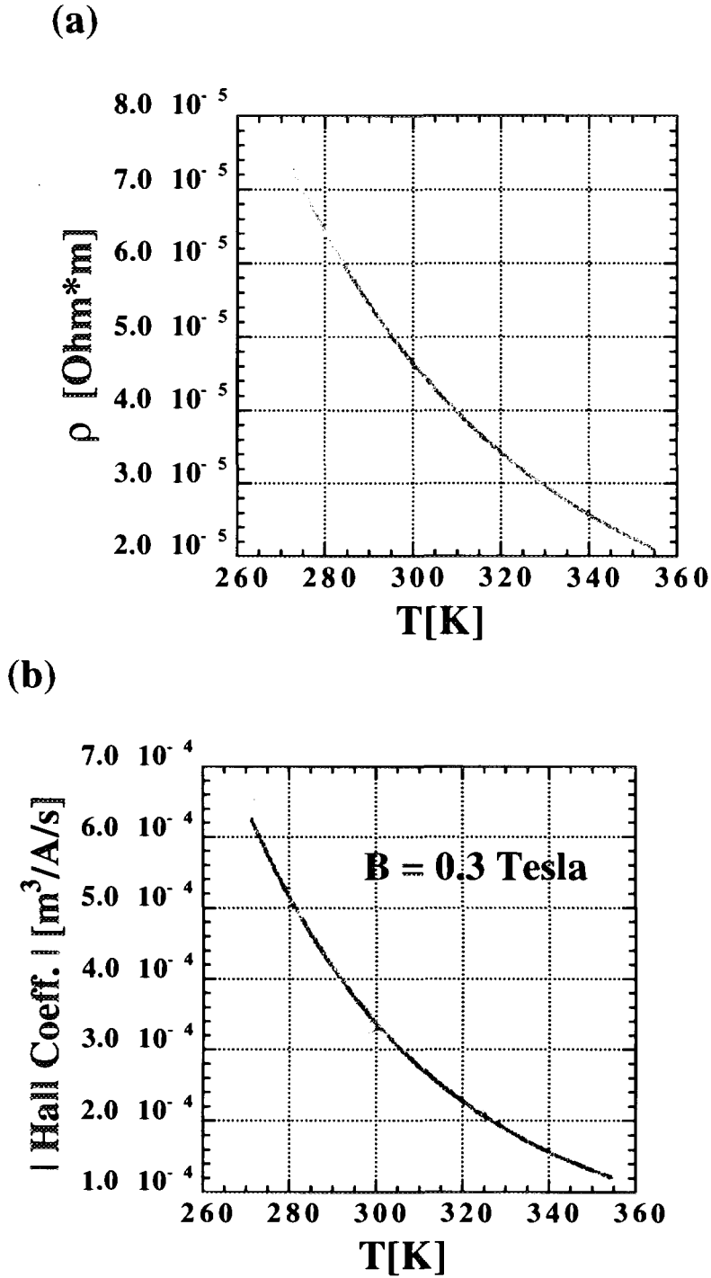
FIG. 3. Resistivity (a) and Hall coefficient (b) of InSb sample as a function of temperature. The closed circles indicate the experimental results. The solid curve is a guide of eyes.
