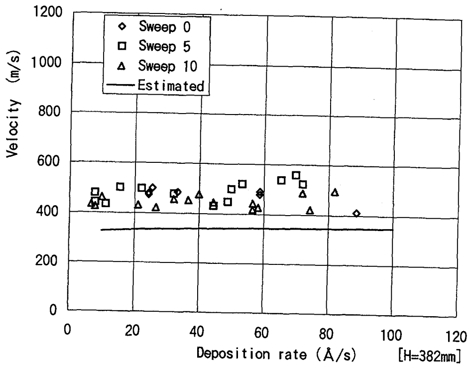
Fig.13 Velocity of Ytterbium atomic beam
