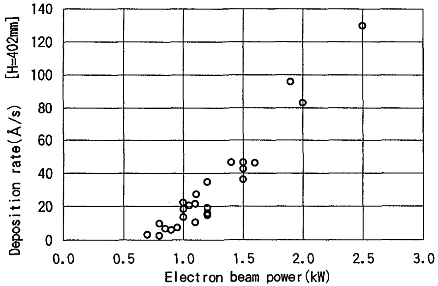
Fig.8 Deposition rate of Neodymium evaporant as a function of electron beam power
