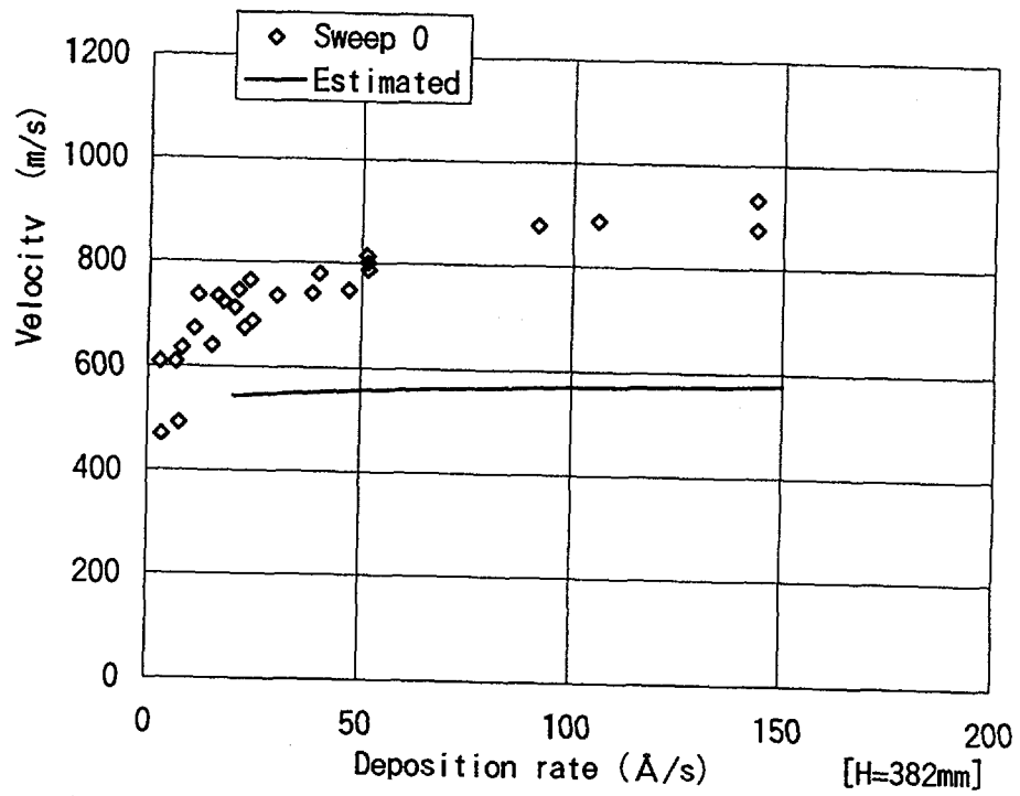
Fig.14 Velocity of Neodymium atomic beam
