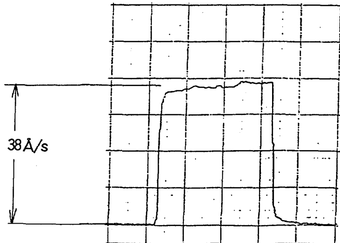
Fig.2 Examples of output signal of vacuum balance and deposition rate measured by a quartz crystal sensor at a height of 402 mm above a crucible (Evaporant: Cerium)
