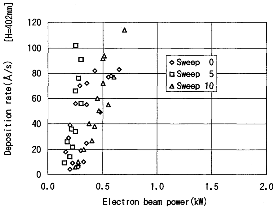
Fig.6 Deposition rate of Samarium evaporant as a function of electron beam power
