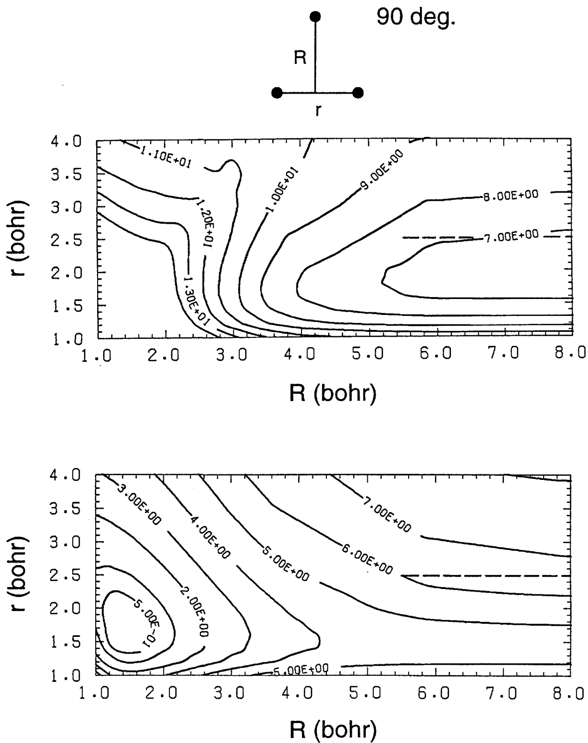
Fig.2 Contour maps of H_3^+ potential energy surfaces for the C_{2v} spatial geometry. The contour for the 1A' ground (first excited) state is shown in the lower (upper) part of the figure. The contour levels are in eV with respect to zero energy which is chosen to be the minimum of the ground state surface. The dashed lines on contours indicate the position where the avoided crossing appears.
