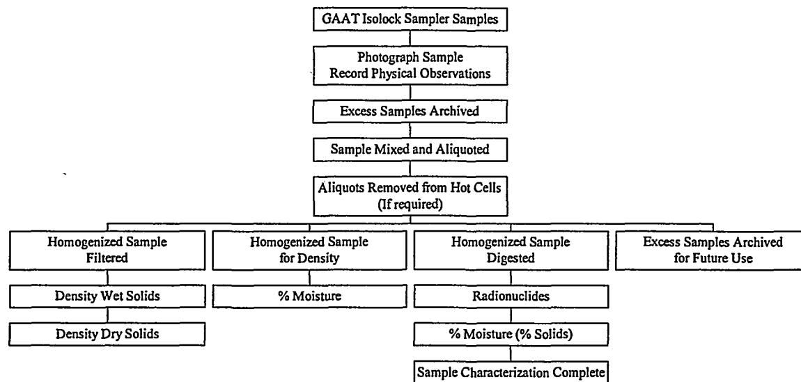
Fig. 1. Overall analysis scheme for the GAAT Isolock Sampler.
