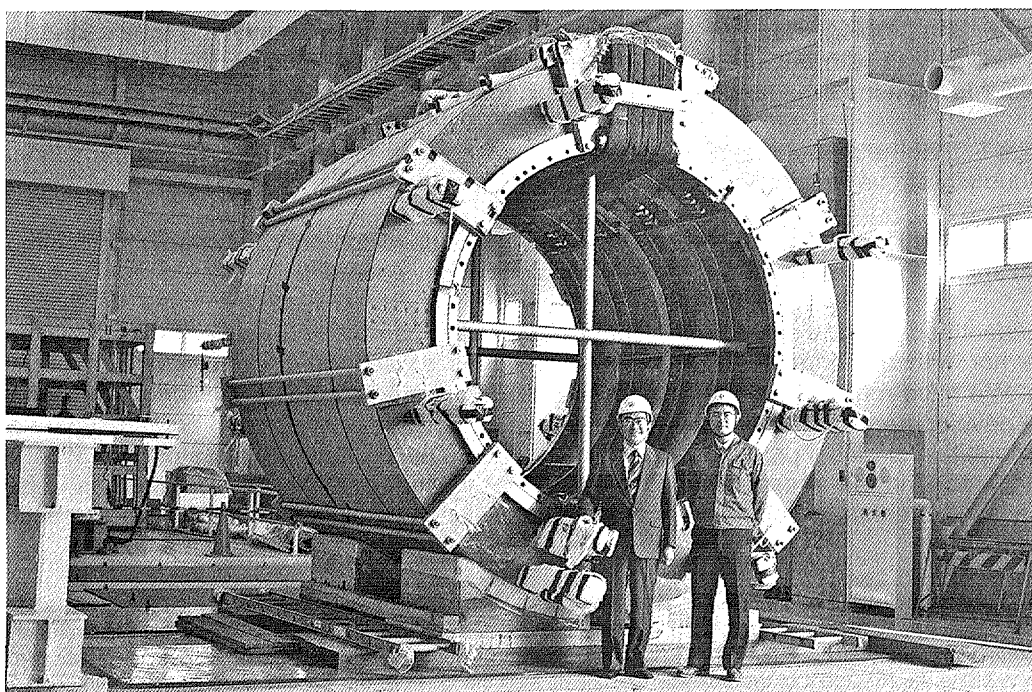
H. Tsuji (Head of JAERI Superconducting Magnet Laboratory) and Co-worker T. Ando in front of the CS Model Coil Outer Module which was delivered to the test site at Naka, JAERI on 11 November 1998.
