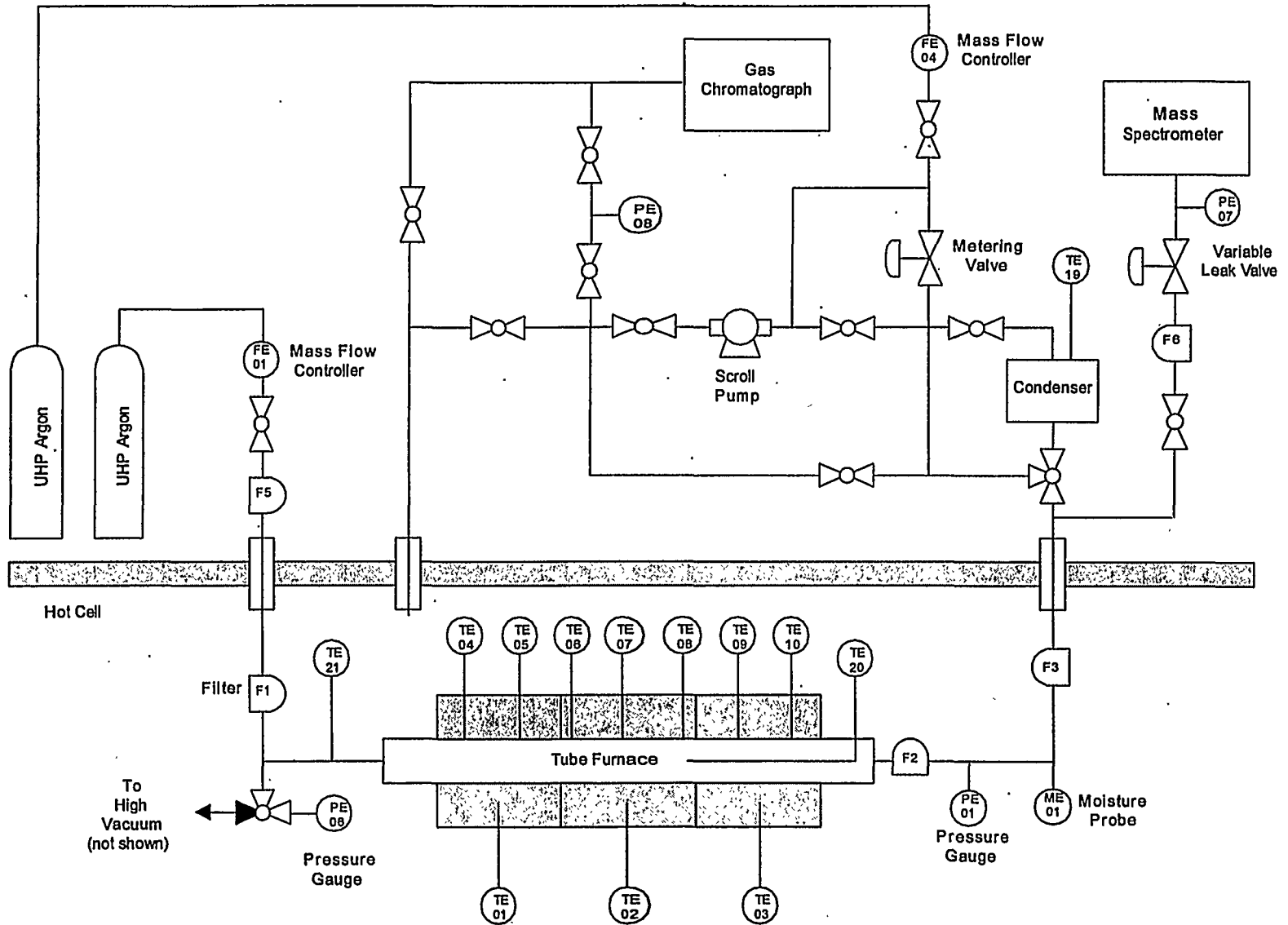
Figure 2.3. Generalized View of the Furnace Testing System
