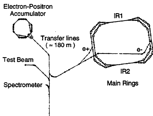
Figure 1: Layout of DAΦNE accelerators and transfer lines.
