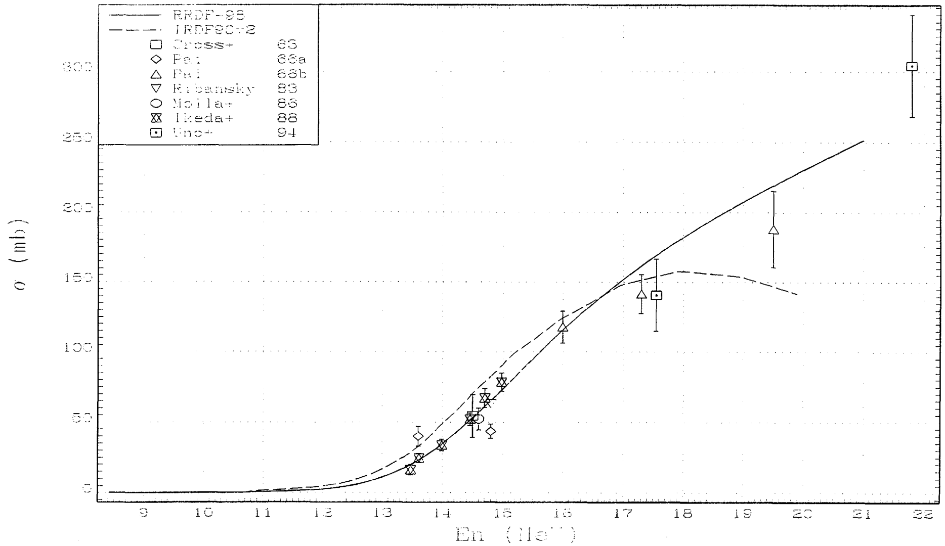
Fig.7. RRDF-98 evaluated excitation function for the ^{47}\text{Ti}(n,x)^{46m+g}\text{Sc} reaction in comparison with IRDF-90 (version 2) curve and experimental data.
