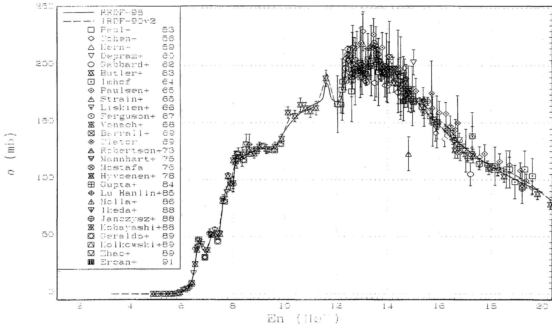
Fig.4. RRDF-98 evaluated excitation function for the ^{24}\text{Mg}(n,p)^{24}\text{Na} reaction in comparison with IRDF-90 (version 2) curve and experimental data.
