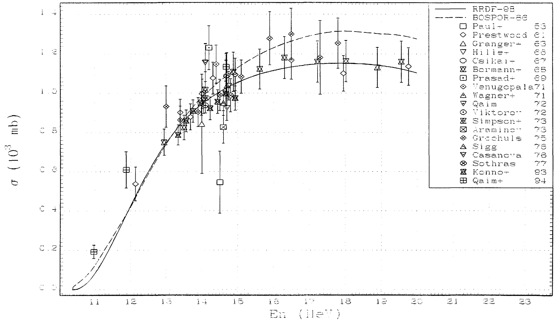
Fig.17. RRDF-98 evaluated excitation function for the ^{75}\text{As}(n,2n)^{74}\text{As} reaction in comparison with BOSPOR-86 curve and experimental data.
