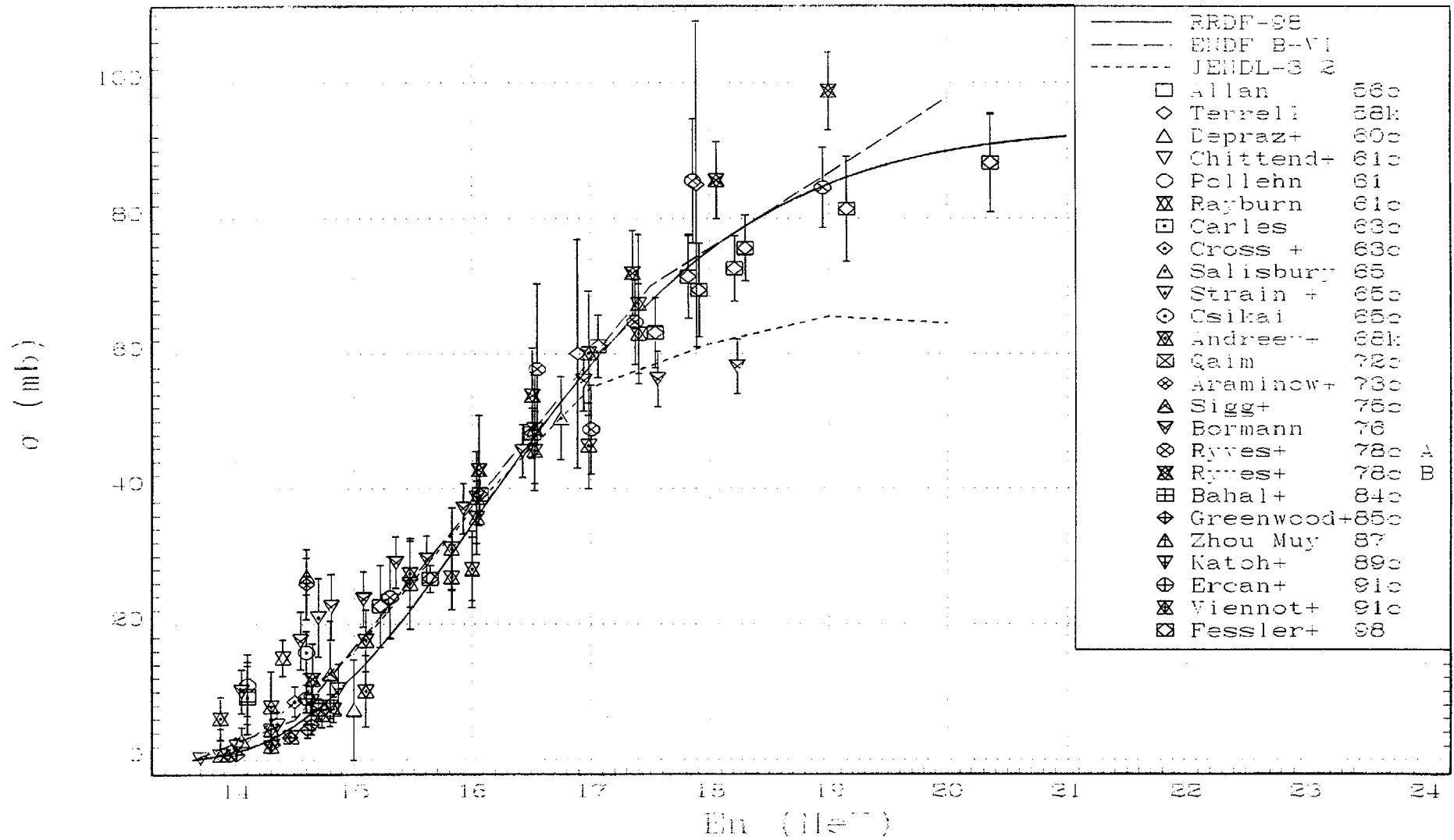
Fig.12. RRDF-98 evaluated excitation function for the ^{54}\text{Fe}(n,2n)^{53m+g}\text{Fe} reaction in comparison with ENDF/B-VI and JENDL-3.2 curves and experimental data.
