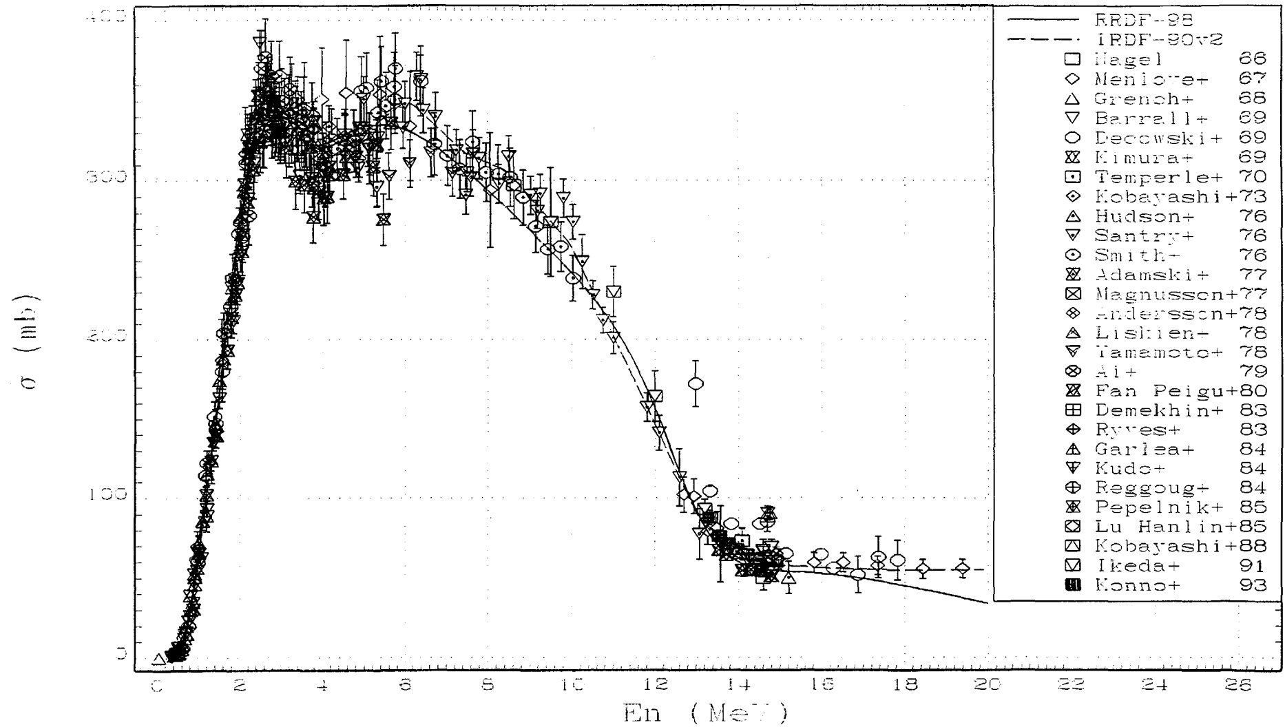
Fig.21. RRDF-98 evaluated excitation function for the ^{115}\text{In}(n,n')^{115m}\text{In} reaction in comparison with IRDF-90 (version 2) curve and experimental data.
