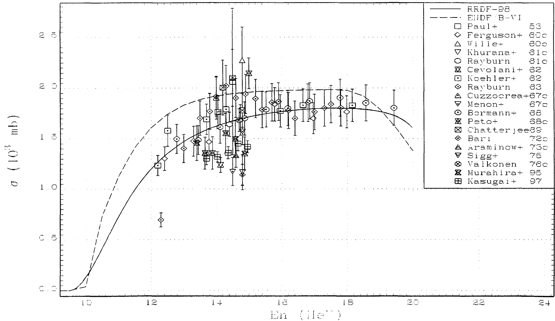
Fig.22. RRDF-98 evaluated excitation function for the ^{141}\text{Pr}(n,2n)^{140}\text{Pr} reaction in comparison with ENDF/B-VI curve and experimental data.
