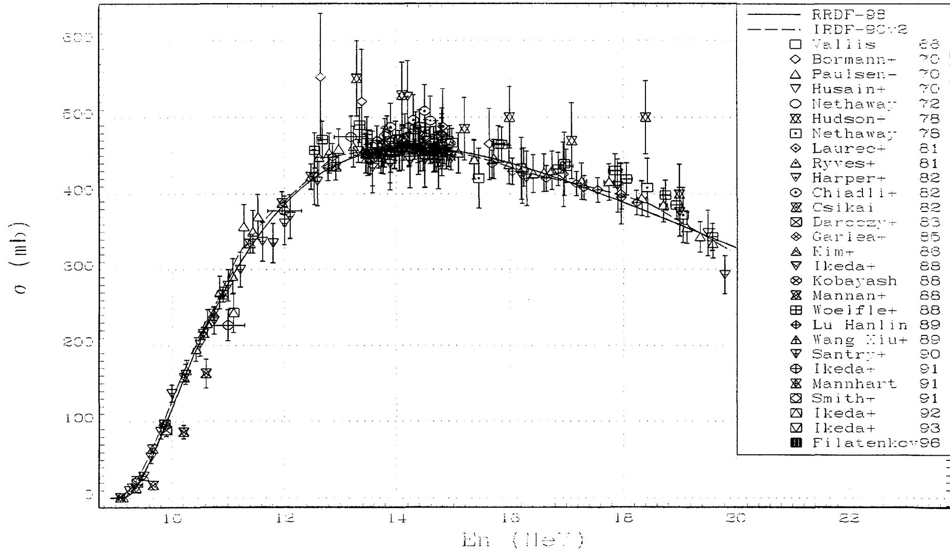
Fig.18. RRDF-98 evaluated excitation function for the ^{93}\text{Nb}(n,2n)^{92m}\text{Nb} reaction in comparison with IRDF-90 (version 2) curve and experimental data.
