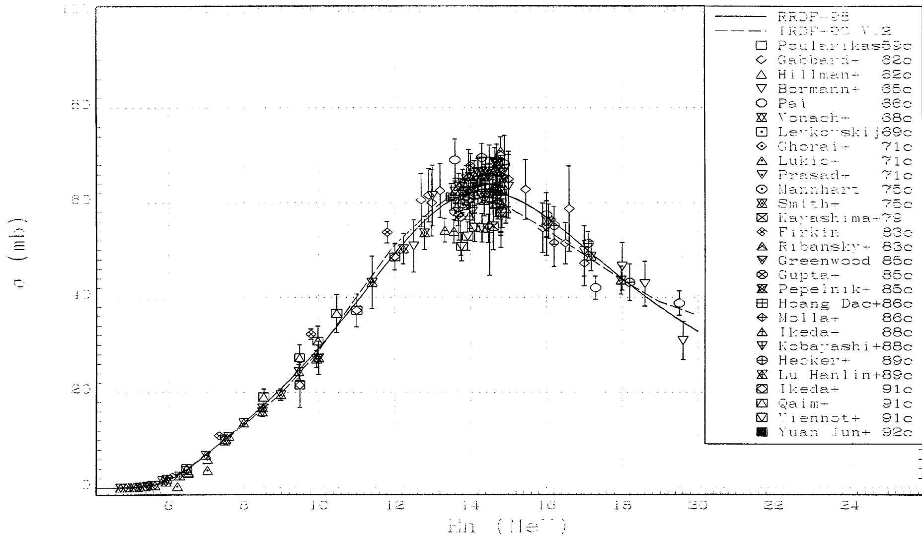
Fig.9. RRDF-98 evaluated excitation function for the ^{48}\text{Ti}(n,p)^{48}\text{Sc} reaction in comparison with IRDF-90 (version 2) curve and experimental data.
