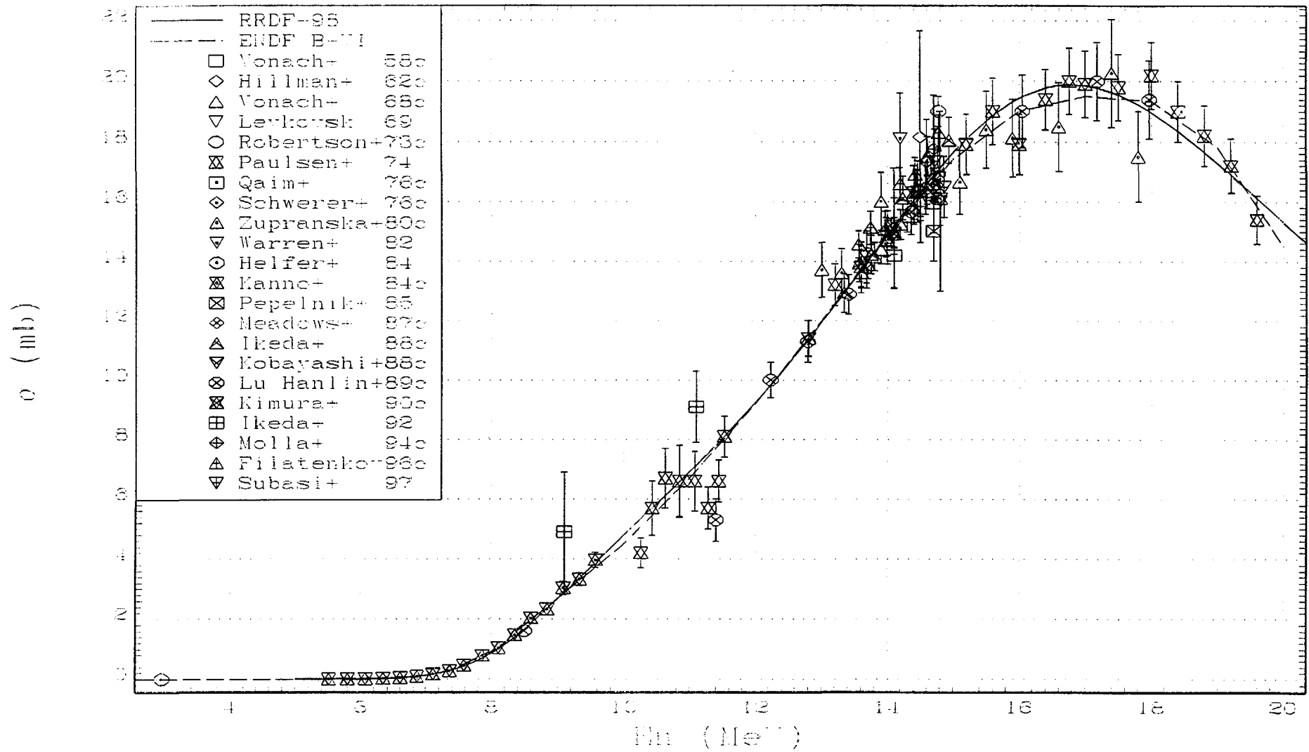
Fig.11. RRDF-98 evaluated excitation function for the ^{51}\text{V}(n,\alpha)^{48}\text{Sc} reaction in comparison with ENDF/B-VI curve and experimental data.
