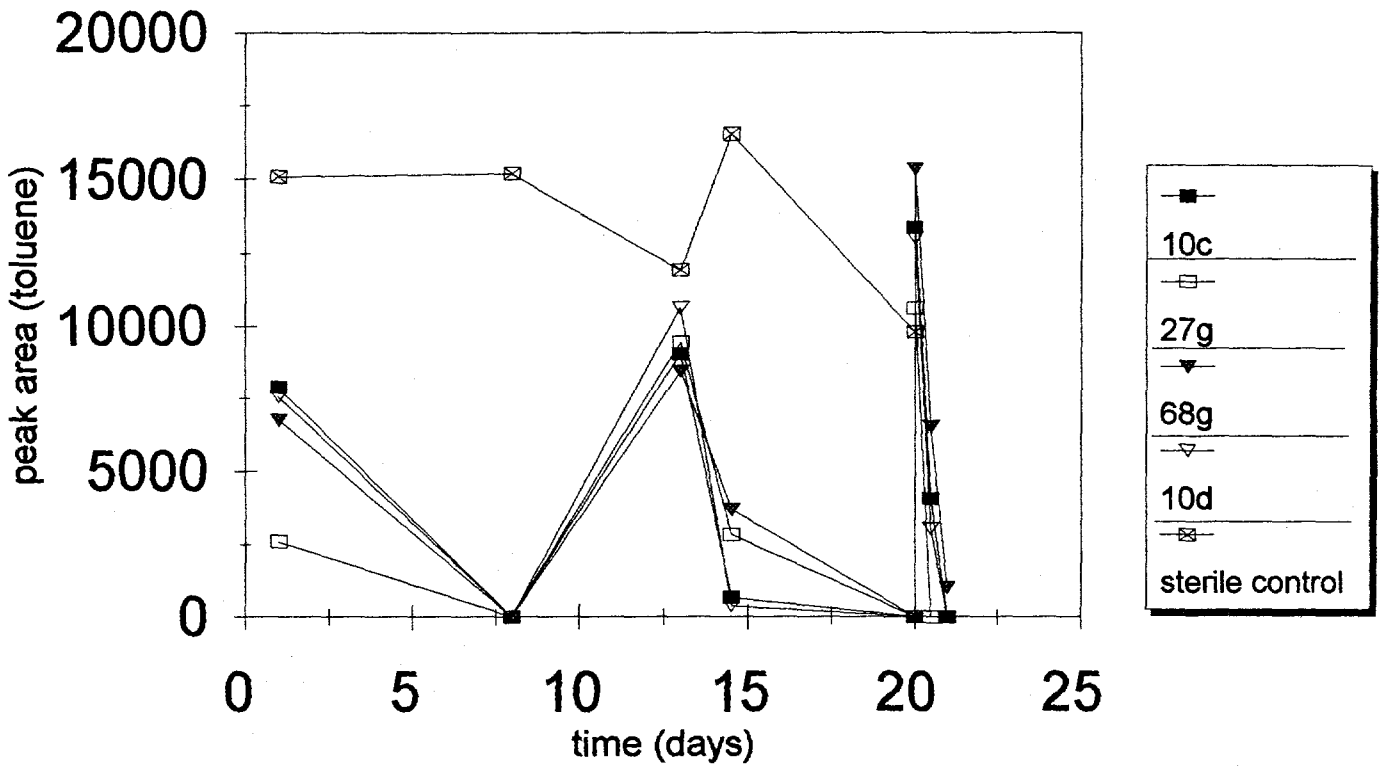
Figure 6. GC analysis of toluene enrichments under denitrifying conditions. 10c through 10d samples are averages of triplicate samples.
