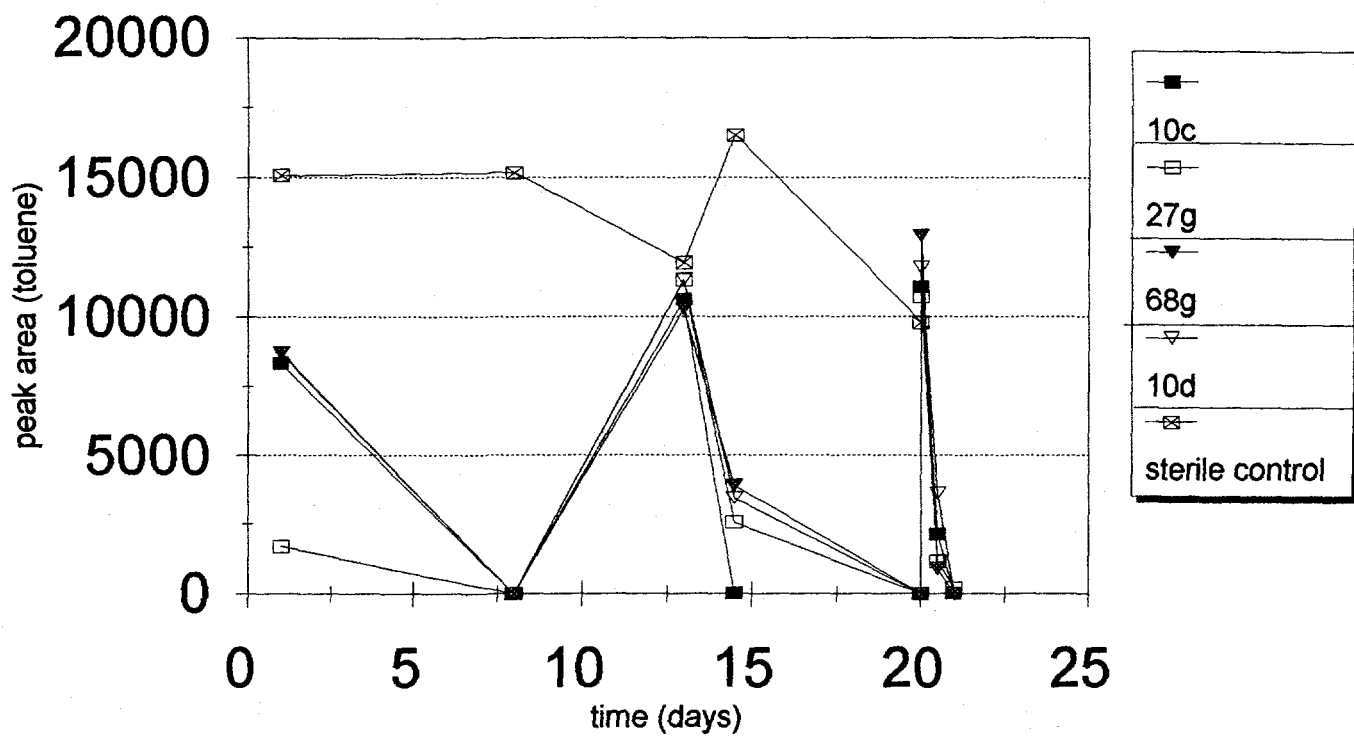
Figure 7. GC analysis of toluene enrichments under sulfate reducing conditions. Samples 10c through 10d are averages of triplicate samples.
