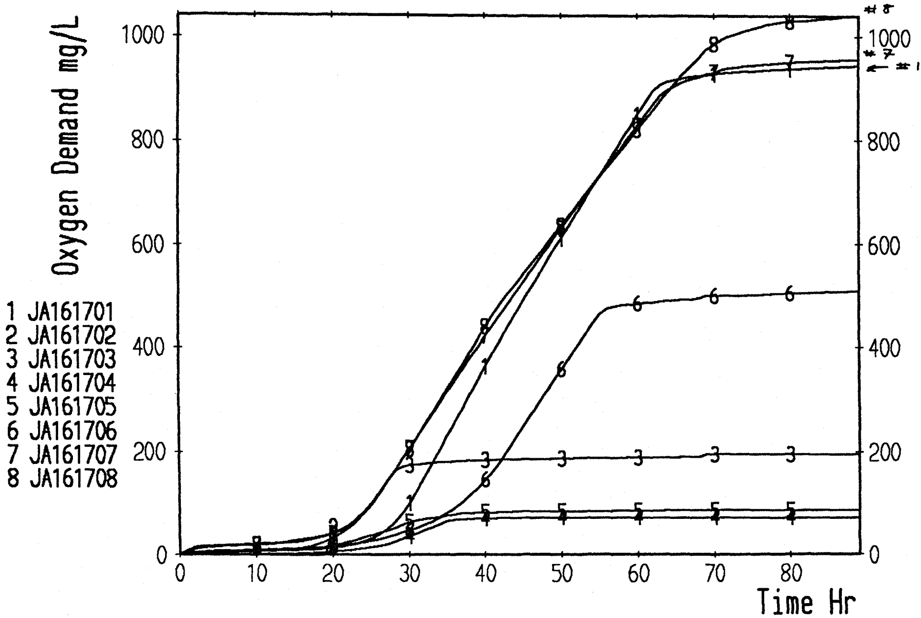
Figure 3. Respirometric data from the initial toluene degradation (A3) experiment. Reactor 1 contains 0.1% glucose (positive control), 3 and 4 contain 20 ppm toluene, 5 and 6 contain 100 ppm toluene and 7 and 8 contain 100 ppm toluene plus 0.1% glucose.
