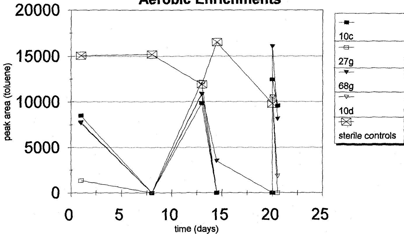
Figure 8. GC analysis of toluene enrichments under aerobic conditions. 10c through 10d samples are single samples and the sterile controls are averages of four sterile samples (10c through 10d).
