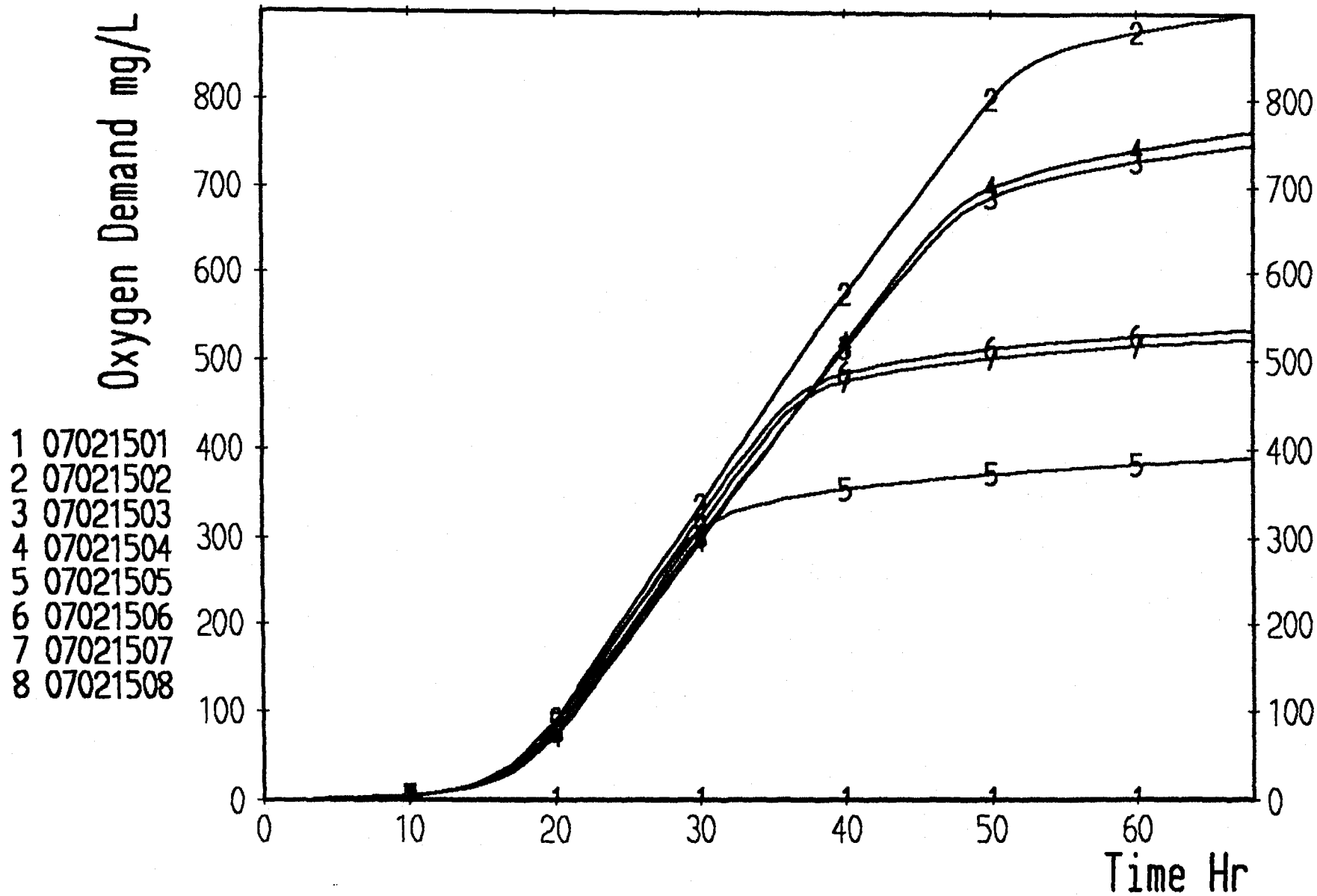
Figure 1. Respirometric data from initial respirometric experiment. Reactor 1 is a negative control, reactors 2-4 are 4 g/L nutrient broth and reactors 5-7 are 2g/L nutrient broth.
