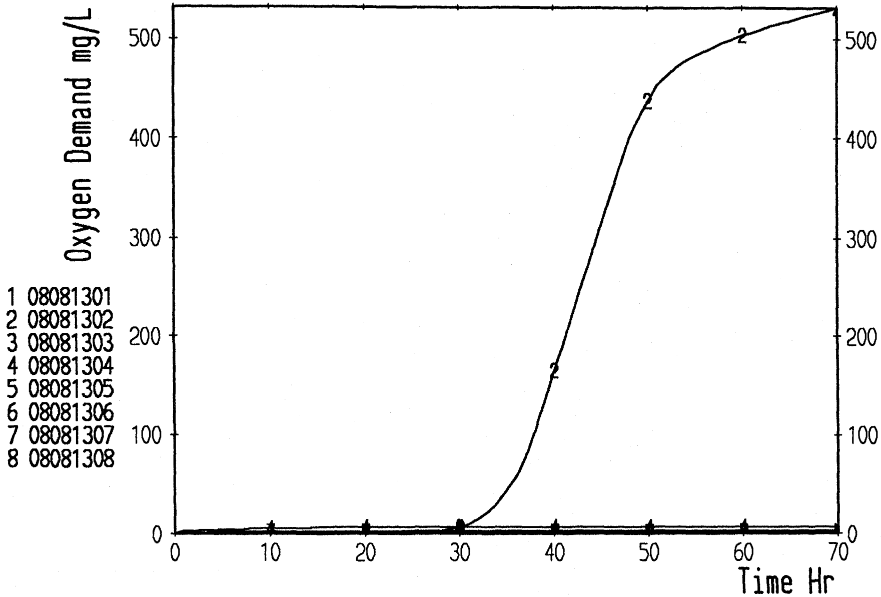
Figure 2. Representative respirometric data from diesel fuel degradation experiments. Reactor 1 contains nutrient broth and 0.1% diesel fuel. Reactor 2 is a positive control containing nutrient broth. Reactor 3 is a negative control containing 0.1% diesel fuel and reactors 4-8 are live samples containing 0.1% diesel fuel.
