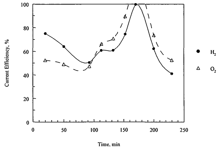
Figure 4.19. Current Efficiencies Based on Hydrogen and Oxygen Generation During Undivided Cell Test With Actual Waste.
