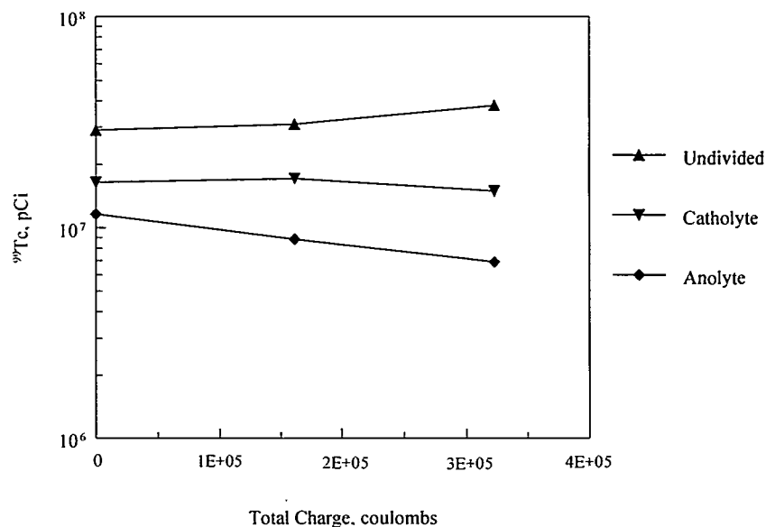
Figure 4.21. Picocuries of 99 Tc in Catholyte, Anolyte, and Undivided Cell Tests With Actual Waste as Functions of Total Charge Passed
