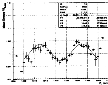
Figure 8: The normalized electron response ( E_e/E_{beam} ) for E = 10, 60, 100 GeV (left column, up to down) and E = 20, 80, 180 GeV (right column, up to down) at \eta = -0.55 as a function of impact point Z coordinate.
