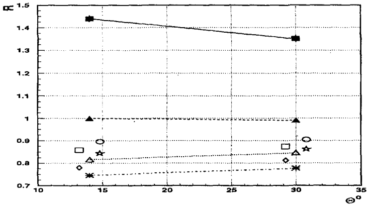
Figure 19: Top: The e/h ratios, the electron and pion responses for the 1m prototype modules as a function of \Theta angle. \blacksquare are the e/h ratios, \blacktriangle are the electron response, the rest is the pion response for 20 ( \diamond ), 50 ( \triangle ), 100 ( \square ), 150 ( \circ ), 300 ( \star ) GeV. Bottom: The e/h ratios, the electron and pion responses for the Module-0 as a function of \Theta angle. \blacksquare are the e/h ratios, \blacktriangle are the electron response, the rest is the pion response for 10 ( \star ), 20 ( \diamond ), 60 ( \triangle ), 80 ( \ast ), 100 ( \square ), 180 ( \circ ) GeV. The lines are the results of linear fits.
