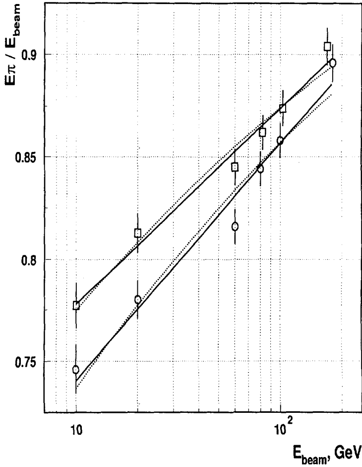
Figure 17: The mean normalized pion response ( E_{\pi}/E_{beam} ) as a function of the beam energy for the Module-0: the \circ points are the \eta = -0.25 data, the \square points are the \eta = -0.55 data. The solid (dashed) lines are the fits of equation (7) with the Wigmans (Groom) parameterization of f_{\pi^0}(E) .
