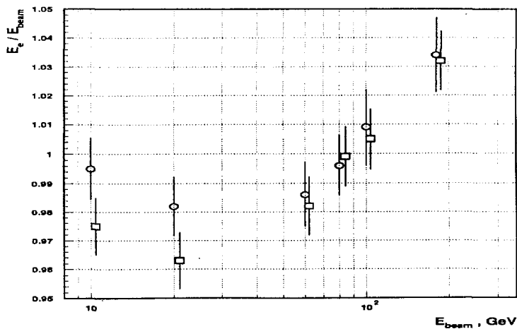
Figure 9: Top: The amplitude (parameter P_1 ) of the electron response as a function of the beam energy. Bottom: The mean normalized electron response as a function of the beam energy. \circ ( \square ) are the data for \eta = -0.25 ( -0.55 ).
