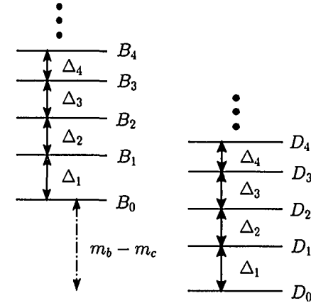
Figure 1: Schematic spectra of the bottom and charmed mesons in the limit m_b, m_c \gg \Lambda_{\text{QCD}} . The offset of the two spectra is not to scale; in reality, m_b - m_c \gg \Delta_i \sim \Lambda_{\text{QCD}} .
