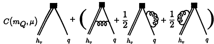
Figure 3: Tree level plus the one-loop renormalization of the current \bar{q}\gamma^\mu\gamma^5 h_\nu in HQET. The double line is the propagator of the effective field h_\nu .
