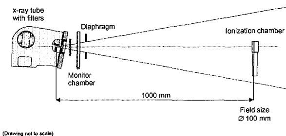
Figure 4. Calibration set-up used at the IAEA Dosimetry Laboratory for the calibration of mammography secondary standards.
