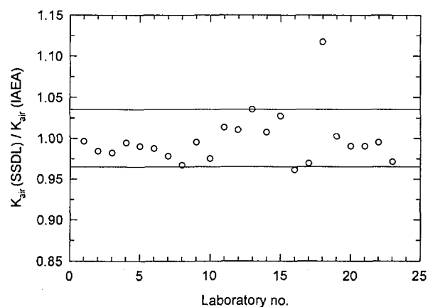
Figure 7. Ratios of the air kerma stated by SSDLs to the TLD measured value at the IAEA Dosimetry Laboratory during the pilot study. The acceptance limit is \pm 3.5\% .
