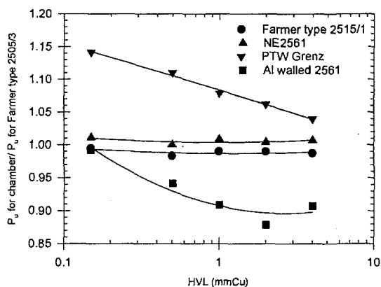
Figure 3 Comparison of perturbation factors.
