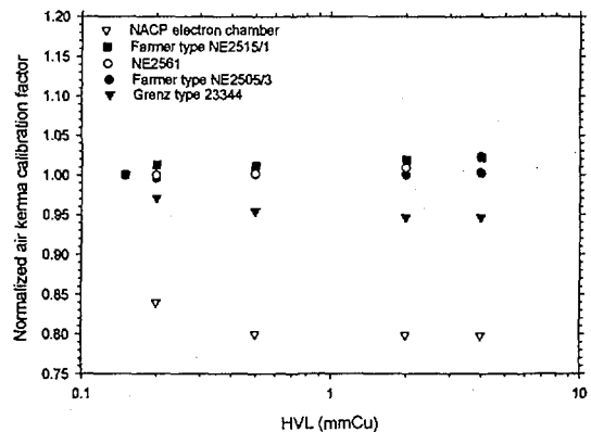
Figure 2b Comparison of the response of ionisation chambers in air
