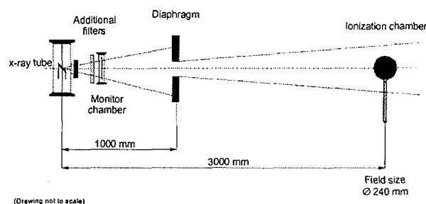
Figure 3. Calibration set-up for ISO x-ray beam qualities at the IAEA Dosimetry Laboratory.
