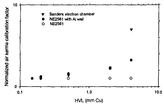
Figure 2a Comparison of the response of the Sanders chamber, a NE2561 with an Aluminium wall and a NE2561 chamber.
