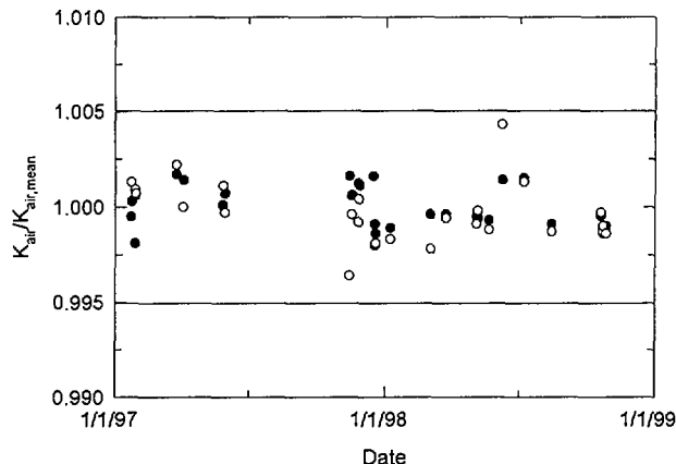
Figure 6. Measured values of the air kerma at the reference point corrected for source decay for the ^{137}\text{Cs} ( \bullet ) and ^{60}\text{Co} ( \circ ) beams of the Buchler OB 85 irradiator.
