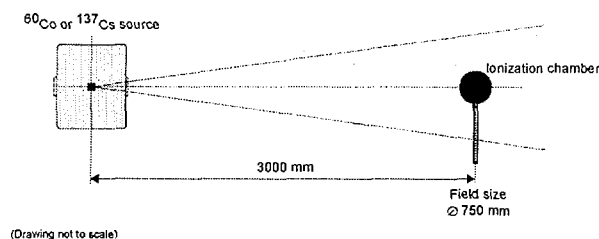
Figure 2. Calibration set-up used at the IAEA Dosimetry Laboratory for the calibration of radiation protection secondary standards in ^{137}\text{Cs} and ^{60}\text{Co} reference gamma ray beams.
