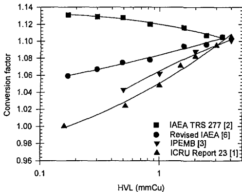
Figure 1 Comparison of the factors to convert the air kerma measured using an ionization chamber to absorbed dose to water at 5 cm depth in water.
