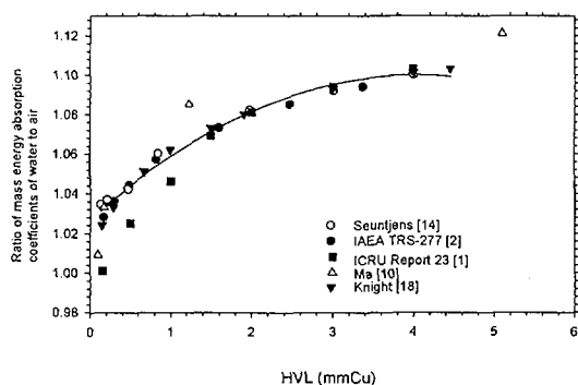
Figure 4: Comparison of the ratio of mass energy absorption coefficients of water to air.
