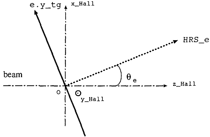
Figure 1: Coordinate system at the target for the lepton arm. The view is in horizontal plane. (X,Y,Z are axis in Hall A frame).
