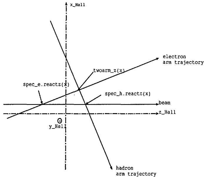
Figure 4: Definition of the vertex variables in Espace.
