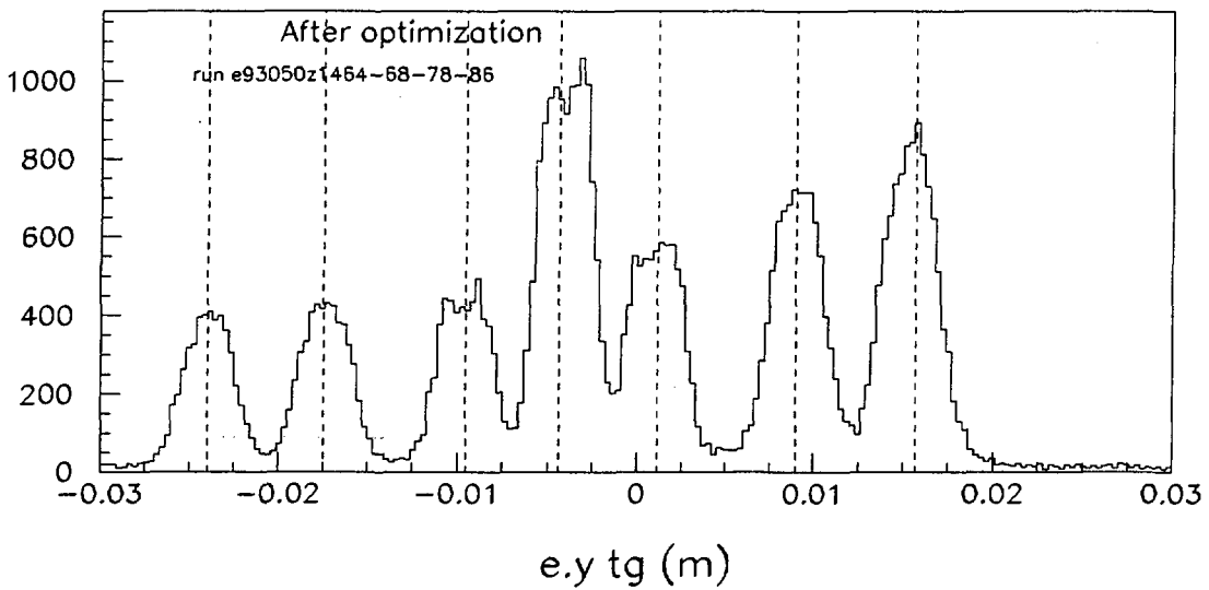
Figure 2: Position for 7 thin targets on y_{tg} axis in electron spectrometer system. The dashed line represents the theoretical position on y_{tg} axis ( = \bar{Y} in the text.)
