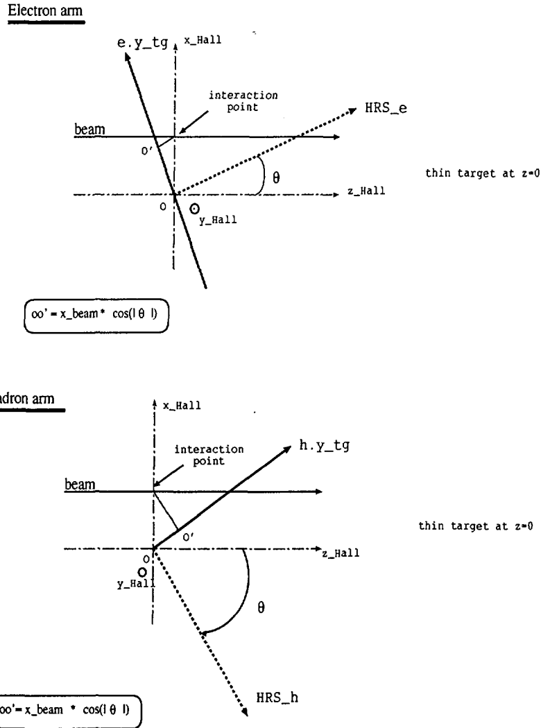
Figure 7: Influence of the beam average position on the y coordinate. O represents the center of spectrometer frame and O' is where the interaction point is seen by the spectrometer.
