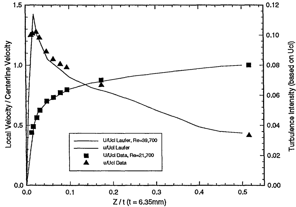
Figure 2. (a) HFA calibration in single-phase liquid flow (b) Single-phase turbulent profiles compared with Lafer's (1951) data
