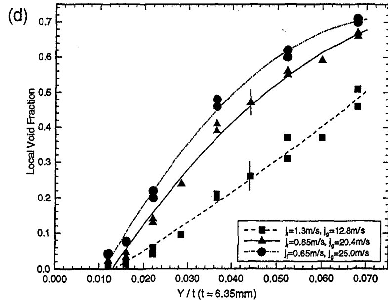
Figure 4. Near-wall HFA data. (a) liquid velocity using calibration (b) interfacial velocity using cross-correlation (c) turbulence intensity (d) void fraction
