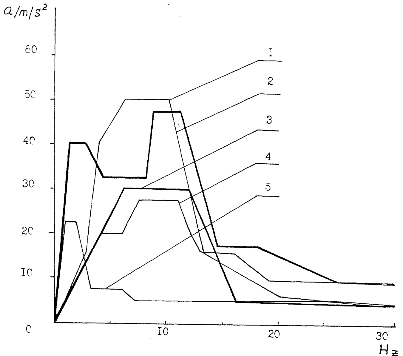
Fig. 5 Envelope floor response spectra. Reactor section. Elevation 36.6 m. Maximum acceleration 0.2g. D=2%. Unified NPP WWER-1000. 1- SIEMENS-Kozloduy-hard soil. 2- AEP-SIEMENS-12 set of accelerogram for soft,soft layered, medium, medium layered and hard soil. 3- AEP-10 set of accelerograms defined by the Academy of Science in 1984-medium soil. 4- For calculation of the reactor and main coolant loops. 5- SIEMENS-Kozloduy-soft soil
