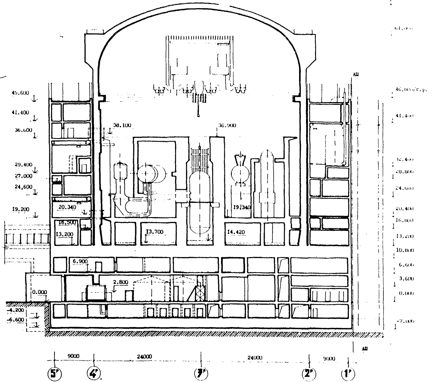
Figure 1 : Section of Building
