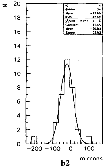
Fig.18. Deviations measured data from nominal dimensions for spacer 9.
