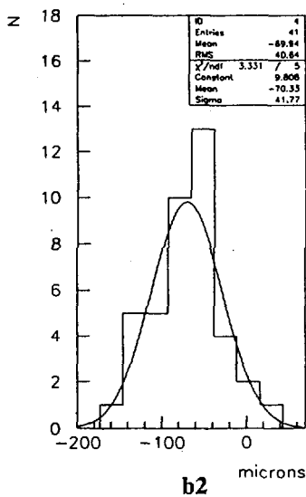
Fig.19. Deviations measured data from nominal dimensions for spacer 10.
