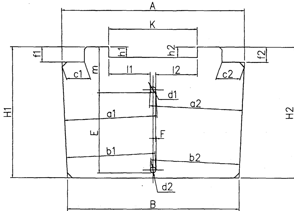
Fig.9. The scheme of spacer #12 measurements.
