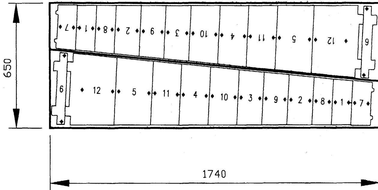
Fig.23. The scheme of packing of spacers sets into boxes.
