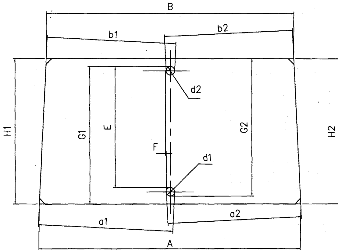
Fig.6. The scheme of spacers measurements.
