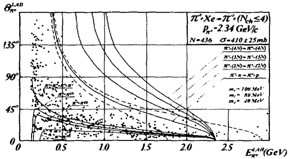
Fig. 7. Same as in Fig. 4 but for all channels of quasi-free \pi^+ +Xe interactions [1,8]. Shown are also different kinematics curved described in the figure.
