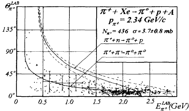
Fig.4. Scatter plot of experimental points for \pi^0 mesons from the reaction \pi^+ + \text{Xe} \rightarrow \pi^0 + p + A at 2.34 GeV/c [1,8]. Two solid curves correspond to kinematics of two-particle reactions pointed in the Figure. Within the two dashed curves comprised should be about 90% experimental points representing \pi^0 mesons from the reaction \pi^+ + n \rightarrow \pi^0 + p when target neutrons oscillate at the temperature of 20 MeV. Crosses mark out the regression curve for experimental points.
