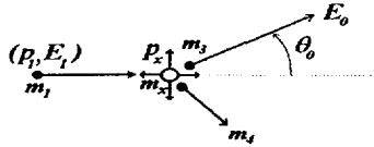
Fig.3. Kinematics of two-body collision with a target particle x 1) at rest and 2) oscillating.
