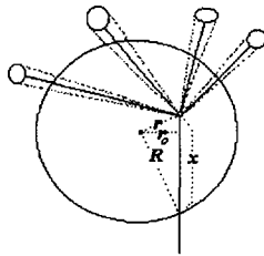
Fig.1. Schematic picture of a quasi-free intranuclear collision.
