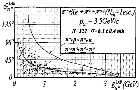
Fig. 6. Same as in Fig.5 but for the reaction pointed in the figure.
