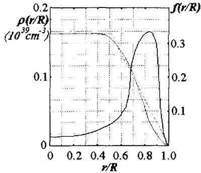
Fig. 2. The probability of quasi-free interactions of \pi^+ mesons with xenon nuclei at 2.34 GeV/c [7].
