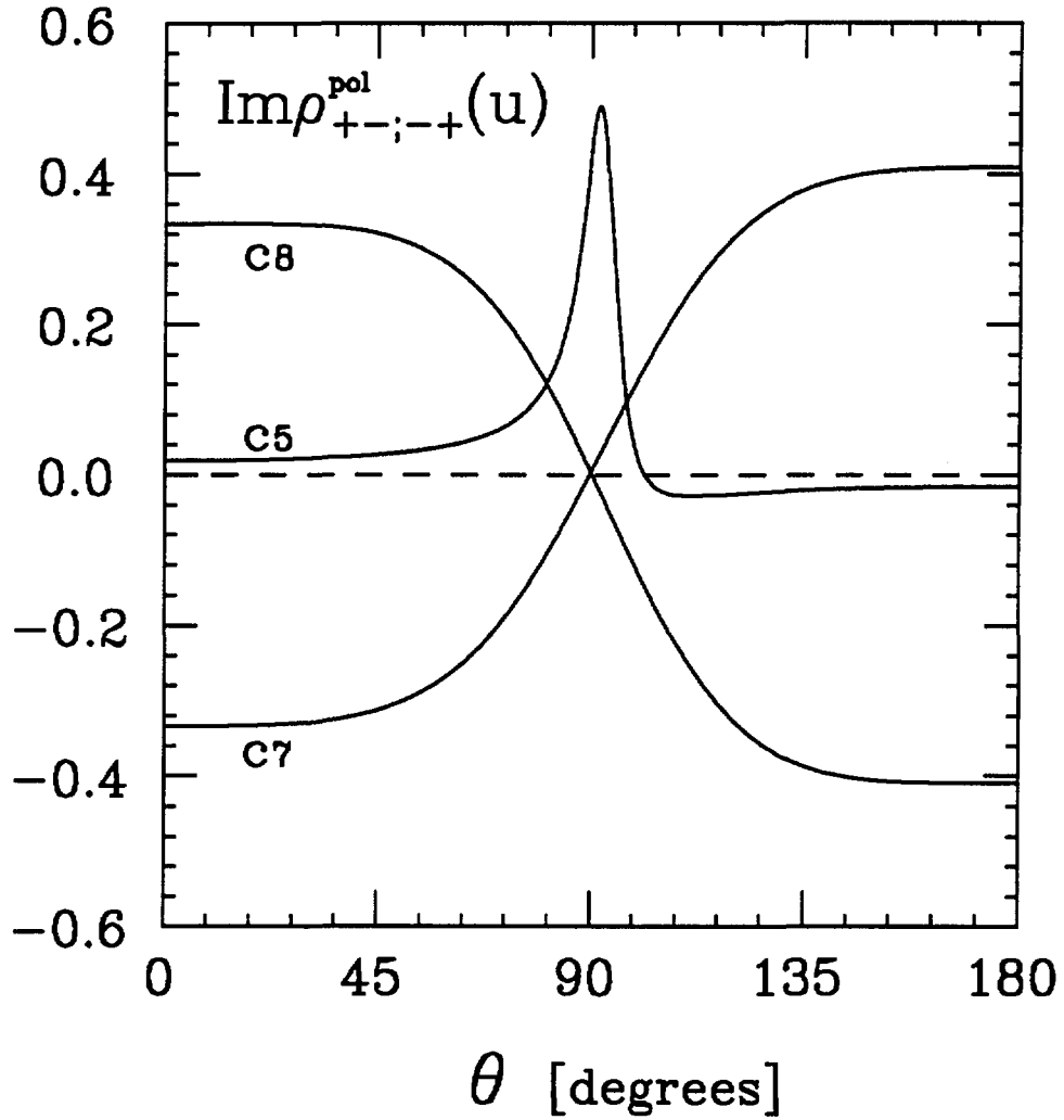
Fig. 3: Plot of \text{Im}[\rho_{+-;-+}^{\text{pol}}(u\bar{u}; \sqrt{s} = M_Z)] as a function of \theta (the production angle of the vector meson in the e^-e^+ c.m. frame) for cases: C5 (both leptons transversely polarized with spins either parallel or anti-parallel); C7 , C8 (both leptons transversely polarized, in different directions). In all other cases, including the unpolarized one, \text{Im}[\rho_{+-;-+}^{\text{pol}}(u\bar{u}; \sqrt{s} = M_Z)] \simeq 0 .
