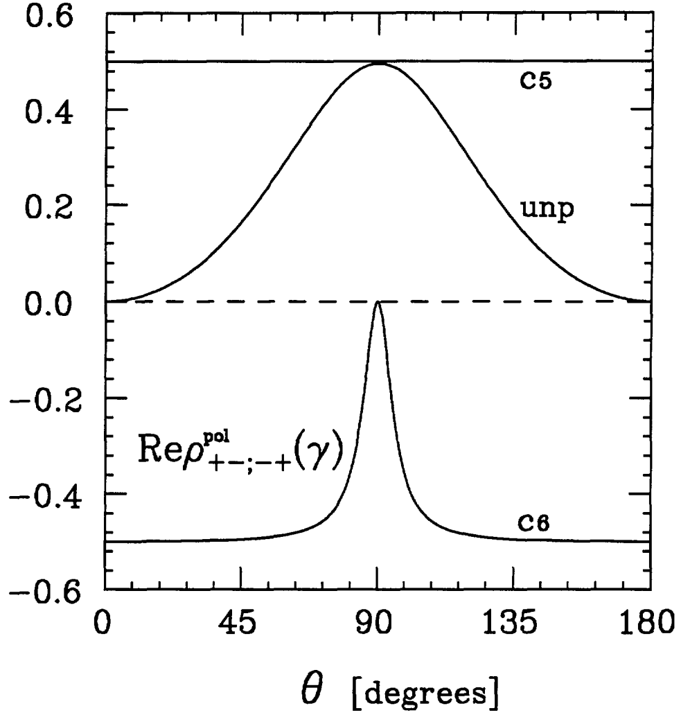
Fig. 5: Plot of \text{Re}[\rho_{+-;-+}^{pol}(q\bar{q}; \sqrt{s} \ll M_Z)] as a function of \theta (the production angle of the vector meson in the e^-e^+ c.m. frame) for cases C5 and C6 (both leptons transversely polarized with spins either parallel or anti-parallel). All other cases give the same result given by unpolarized leptons, which is shown for comparison. Quark masses have been taken into account, with \epsilon = 2m_q/\sqrt{s} = 0.1 .
