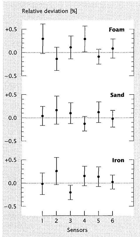
Figure 1 Relative deviation (P_{\text{Umeasured}} - P_{\text{Udeclared}})/P_{\text{Udeclared}} as measured with the TIA method for the foam, sand, and iron matrices. The (1 - \sigma) error flags show the reported uncertainty.
