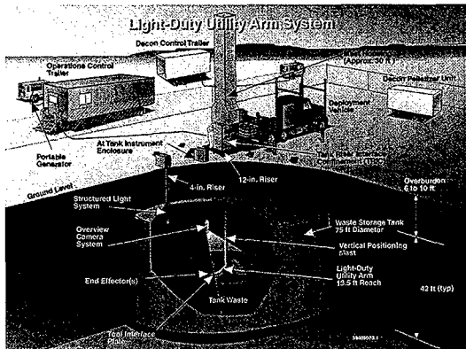
Figure 1 LDUA System
