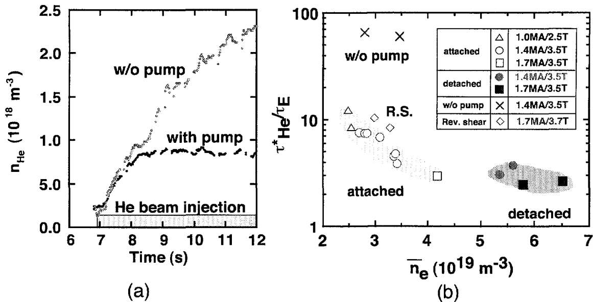
FIG. 13. (a) Temporal change of the helium density in the plasma in comparison between the cases with and without helium pumping during a long helium beam injection into an ELMy H-mode discharge, (b) the ratio of the effective helium pumping time to the energy confinement time as a function of the line-averaged electron density for ELMy H-mode discharges and reversed shear discharges.
