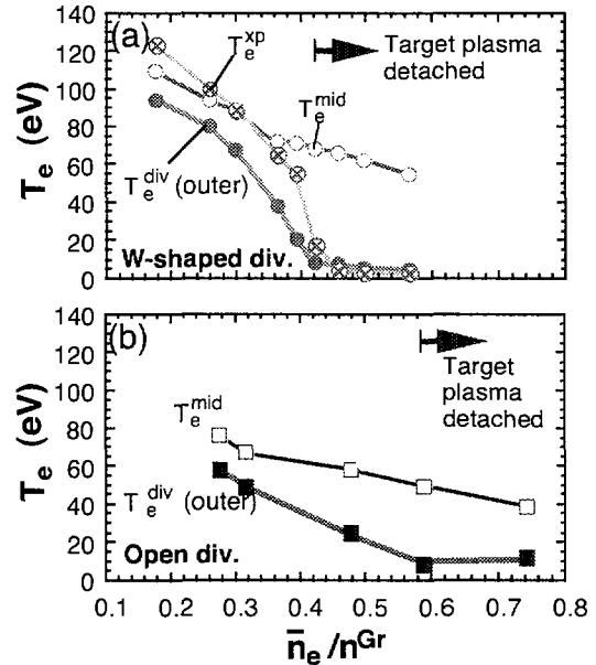
FIG.12. Comparison of the electron temperature in SOL plasma at midplane, near x-point and at outer divertor target: (a) the W-shaped divertor and (b) the open divertor, along with density regions where MARFE is observed.
