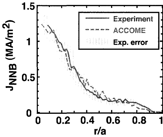
FIG. 15. Comparison of the N-NBI driven current density profile between measurement and ACCOME code calculation: I_p=1.0 MA, B_t=3.5 T and P_{N-NB}=3.7 MW.
