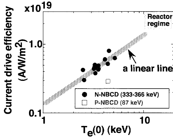
FIG. 16. Current drive efficiency of the N-NBI as a function of the central electron temperature in comparison with P-NBI.
