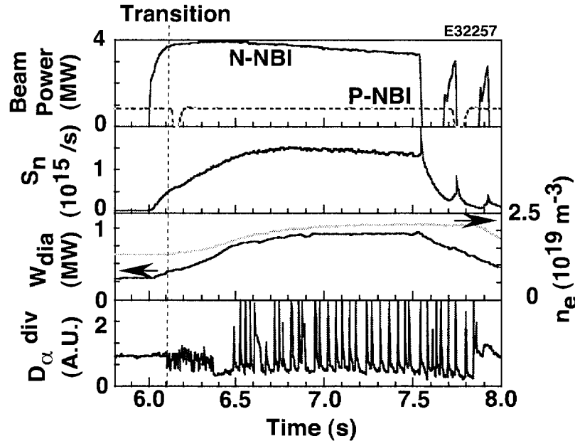
FIG. 14. Waveforms of N-NBI and P-NBI power, neutron emission rate, stored energy, electron density and D_\alpha emissions from a divertor region, showing an H-mode transition induced by N-NB injection at a target electron density of \bar{n}_e \sim 1.3 \times 10^{19} \text{ m}^{-3} for a discharge with I_p = 1 \text{ MA} and B_t = 2.1 \text{ T} .
