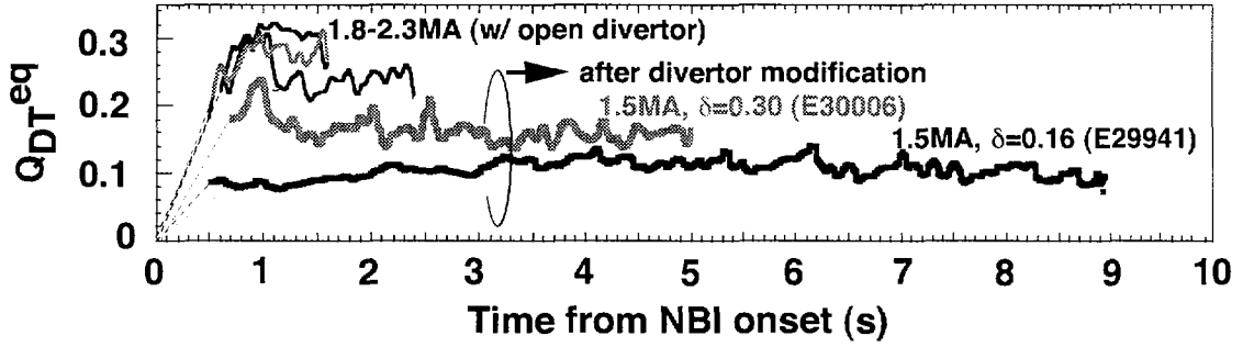
Fig. 8. Time traces of Q_{DT}^{eq} values for high- \beta_p ELMy H-mode discharges, where the discharges with the W-shaped divertor in comparison with the discharges with the open divertor.
