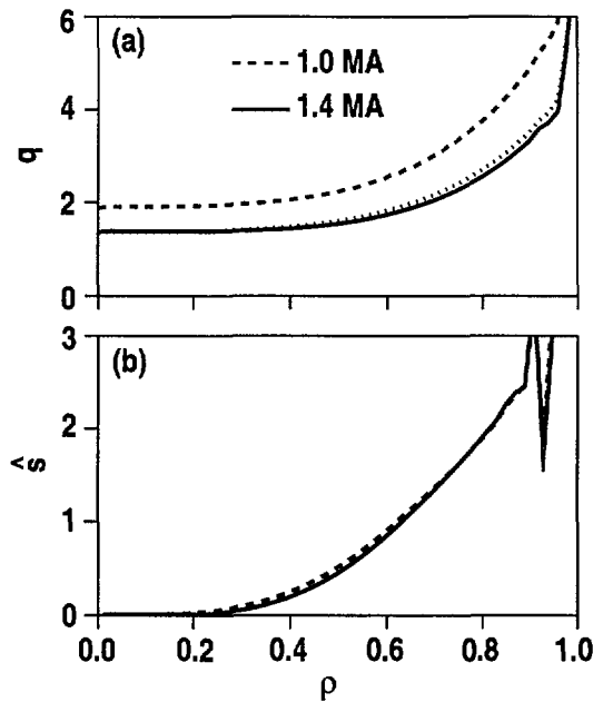
FIG. 1. Radial profiles of (a) safety factor, and (b) magnetic shear for H-mode discharges. The dotted line in (a) represents the 1.0 MA profile scaled to 1.4 MA.
