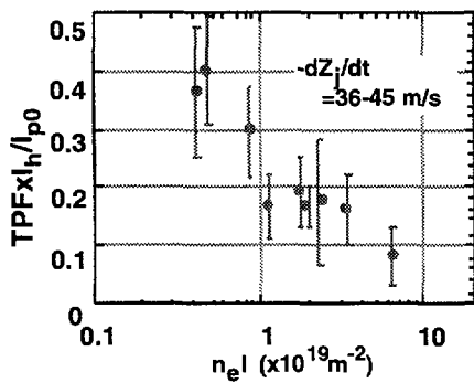
Fig. 6. The TPF \times I_h/I_{p0} versus line integrated electron density ( n_e l ) at the time of the maximum halo current for a vertical shift velocity ( -dz_j/dt ) of 36-45 m/s.
