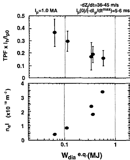
Fig. 5. Relation between TPF \times I_h/I_{p0} , n_e l and the stored energy just before the energy quench ( W_{dia}^{e.q.} ). The stored energy is varied by changing the NB heating power for a fixed plasma current of 1 MA.
