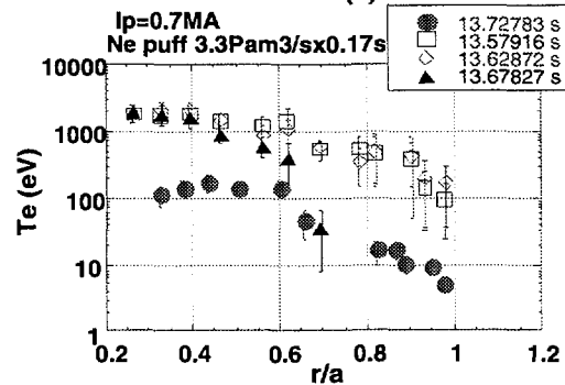
Fig.8. Distribution of the electron temperature measured by YAG Thomson scattering at every 50 ms during neon puffing discharge.
