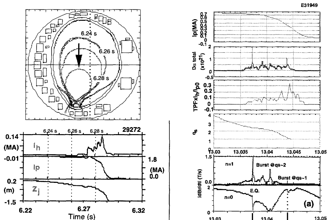
Fig. 1. Waveforms of the halo current during a simulated VDE. A plasma is shifted downward actively to simulate VDE. The dotted line in the upper figure indicates the line of sight of FIR measurement. Halo current starts to flow from t = 6.265 s and reaches its maximum at t = 6.286 s.
