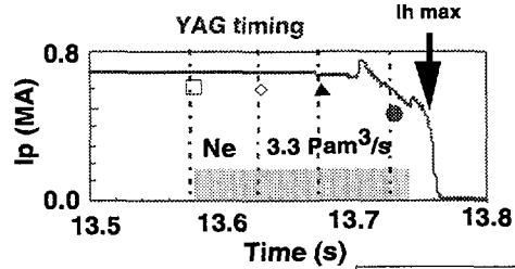
Fig. 7. Wave forms of halo current with ( 3.3 \text{ Pam}^3/\text{s} \times 0.17 \text{ s} ) and without neon gas puffing.
