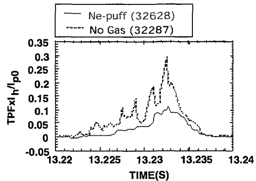
Fig. 7. Wave forms of halo current with ( 3.3 \text{ Pam}^3/\text{s} \times 0.17 \text{ s} ) and without neon gas puffing.
