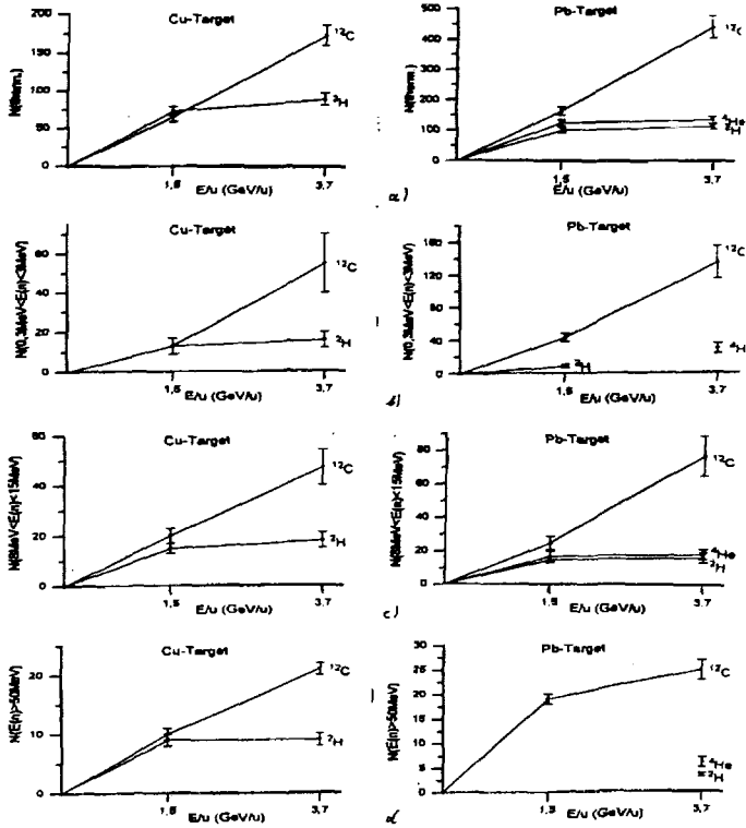
Fig. 7 Experimentally observed neutron numbers in different energy intervals using Cu- and Pb-targets irradiated at the Synchrophasotron
