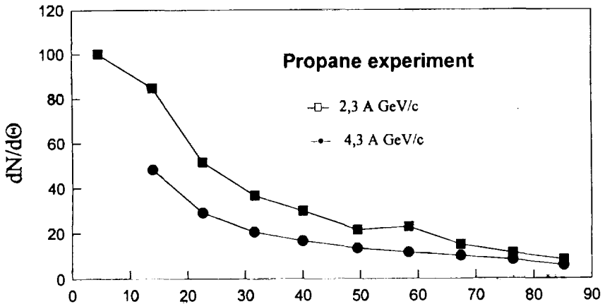
Fig. 14 (and Table 4): The angular distribution of fast ( > 1 \text{ GeV} ) secondary protons produced by 15.1 GeV and 41.5 GeV ^{12}\text{C} , respectively. The 'drawing' gives the results for momentum measurements, the 'Table 1' right side - the results for effectiveness to produce ^{24}\text{Na} in Cu.
