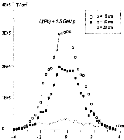
Fig. 5 The beam profile of the Synchrotron beam, measured with SSNTD at our target system
