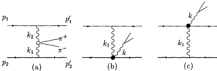
Figure 1: Diagrams for the pion pair production in e and \bar{p} collisions.
