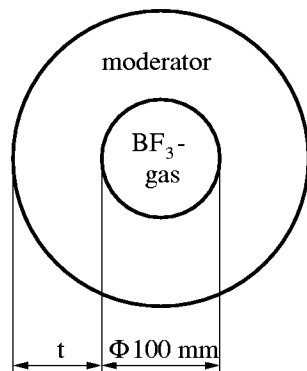
Figure 7: Spherical detector geometry
