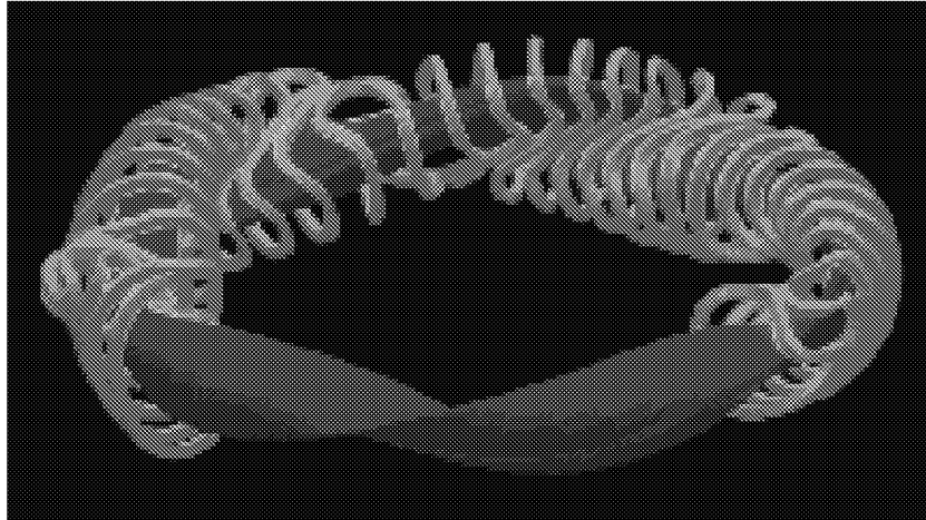
Figure 31: Computer drawing of some modular coils and plasma of W7-X. The five toroidal field periods will maintain the plasma such that it is bean shaped at the corners of the pentagon [2, 1].
