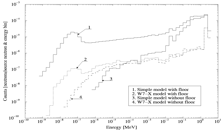
Figure 9: Neutron spectra of the two torus models with and without floor given as the number of neutrons per source neutron and energy bin at the detector position and as function of energy. There are 5 energy bins per decade.
