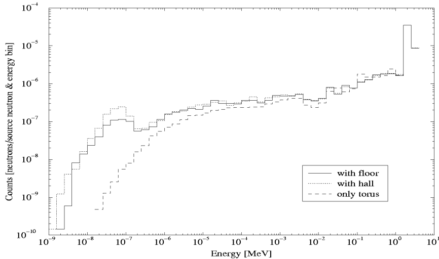
Figure 10: Neutron spectra of the W7-X torus alone, with the floor and with the reactor hall (i.e. floor, walls and ceiling) given as the number of neutrons per source neutron and energy bin at the detector position and as function of energy. There are 5 energy bins per decade.
