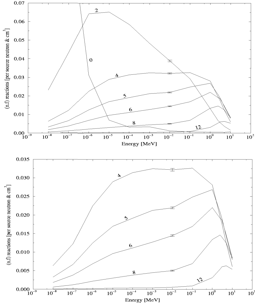
Figure 14: (n,f) reaction rate of polyethylene moderating ^{235}\text{U} as function of incident neutron energy for different moderator thicknesses given in cm. The average relative error in the calculations is about 1.5 %. The lower picture shows only a few of the response curves in order to get a better separation in the high energy interval.
