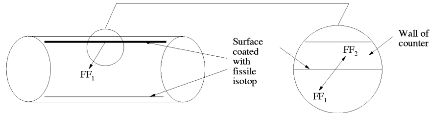
Figure 30: A fission chamber. The interior surface of the detector is coated with a fissile isotope. When fission takes place, the fission fragments, FF_1 and FF_2 , are emitted in opposite directions. One stops in the wall and the other is ionized and detected [9].
