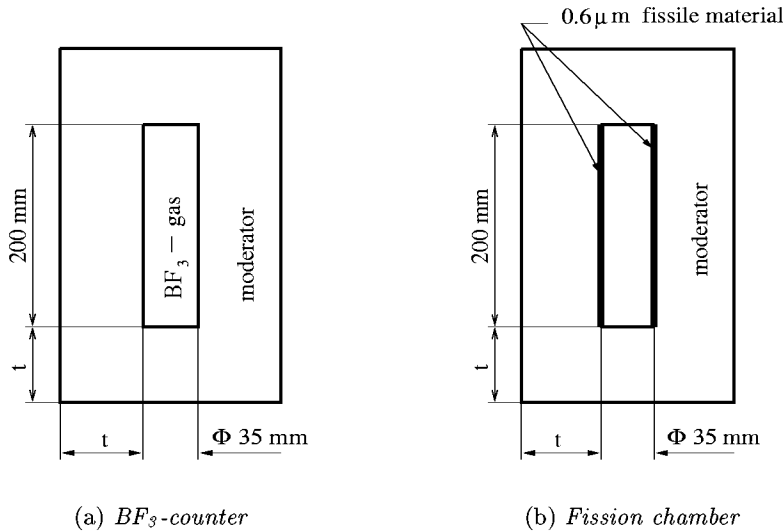
Figure 6: Cylindrical detector geometry
