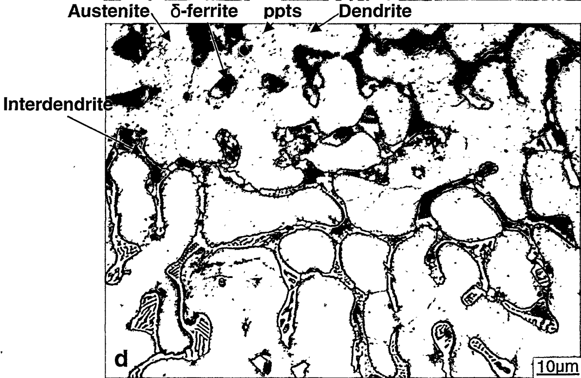
FIGURE 10. (Continued) Optical micrographs of the surface of NOREM 02 WE after EPR testing: (a) as-deposited microstructure for coupon 2-1 (Mag=500X), (b) as-deposited NOREM 02, coupon 2-1 (Mag=1000X), (c) 1150 SR NOREM 02, coupon 2A-1 (Mag=1000X), and (d) 1625 SR NOREM 02, coupon 2B-1 (Mag=1000X). The NOREM 02 EPR coupons were machined from deposits made on Type 304 stainless steel.
