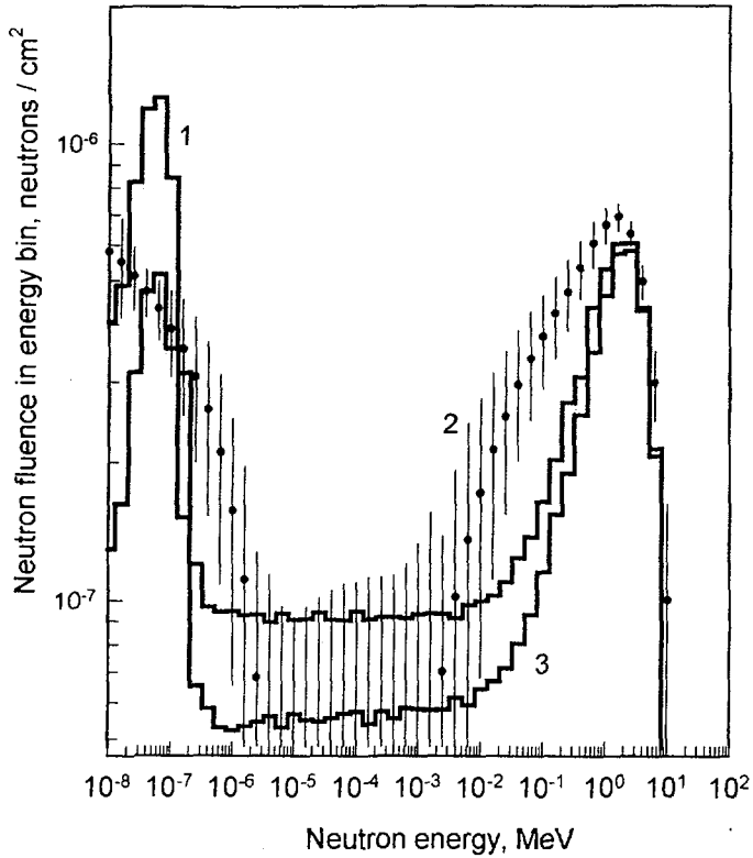
Fig 1. The neutron spectra of the fields free in air and in the calibration room from ^{252}\text{Cf} source (with yield 1 \text{ n}\cdot\text{s}^{-1} ) placed at the centre of polyethylene spheres with diameter 12.7 cm.
