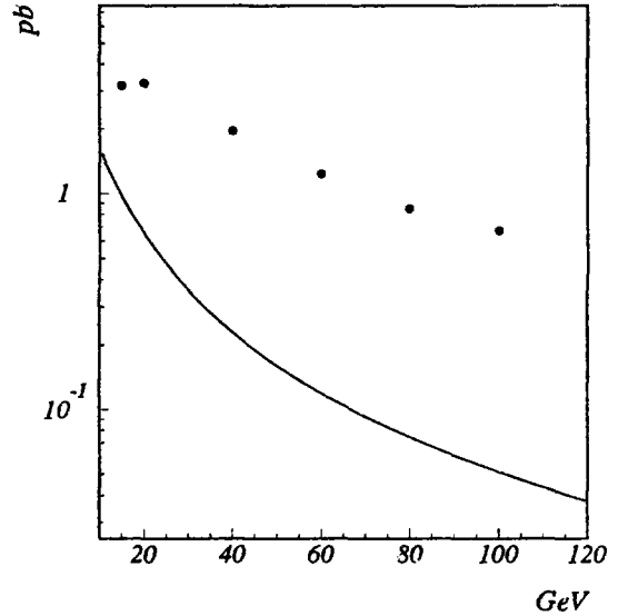
Fig. 4. The gluonic production cross section of \Xi_{cc}^{(*)} ( \bullet ) in comparison with the predictions of the fragmentational mechanism (solid line).
