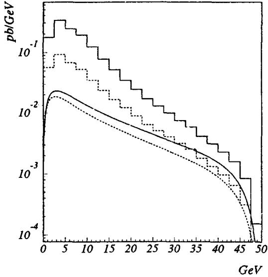
Fig. 2. The distributions over the transverse momentum in the gluonic production of \Xi'_{bc}(\Xi_{bc}^{(*)}) in comparison with the fragmentation result at the interaction energy of 100 GeV.
