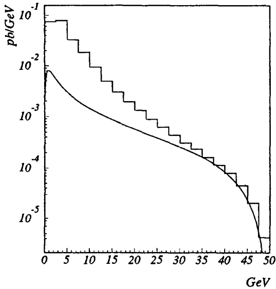
Fig. 5. The distribution over the transverse momentum in the gluonic production of \Xi_{cc}^{(*)} in comparison with the fragmentation result at the interaction energy of 100 GeV.
