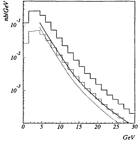
Fig. 3. The differential cross section d\sigma/dp_T of the \Xi'_{bc}(\Xi_{bc}^{(*)}) production in p\bar{p} collisions versus the transverse momentum of the \Xi'_{bc}(\Xi_{bc}^{(*)}) -baryon at the hadron interaction energy of 1.8 TeV, in comparison with the fragmentation result.
