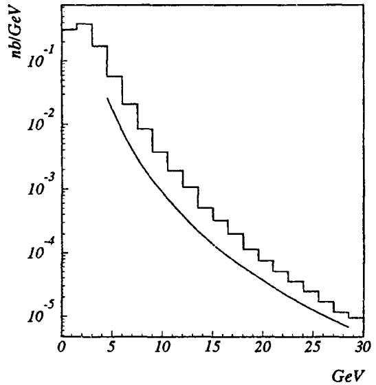
Fig. 6. The differential cross section d\sigma/dp_T of the \Xi_{cc}^{(*)} production in p\bar{p} collisions versus the transverse momentum of the \Xi_{cc}^{(*)} -baryon at the hadron interaction energy of 1.8 TeV in comparison with the fragmentation result.
