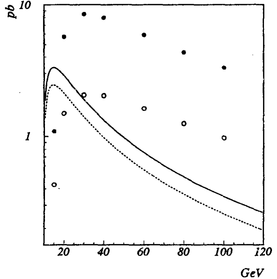
Fig. 1. The gluonic production cross sections of \Xi'_{bc} (o) and \Xi_{bc}^{(*)} (•) in comparison with the predictions of the fragmentational mechanism for \Xi'_{bc} (dashed line) and \Xi_{bc}^{(*)} (solid line).
