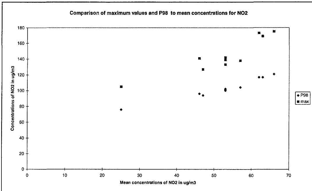
Figure 5: Graphical representation of relationship between maximum values and the 98 th percentiles (P98) and mean concentration of PM 10 and NO 2 for the selected grid squares.
