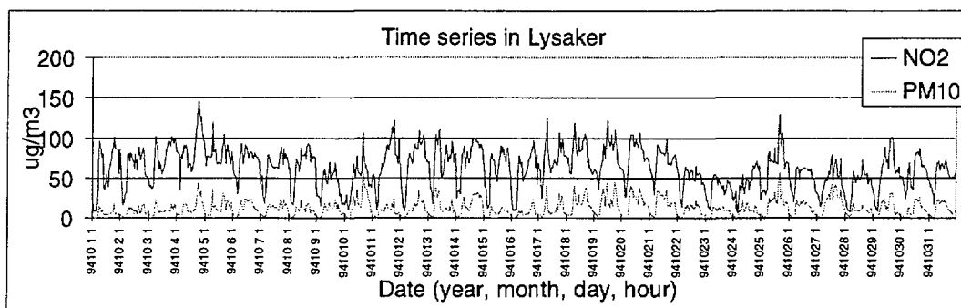
Figure 4: Time series of \text{NO}_2 and \text{PM}_{10} for October 1994 at Lysaker 1 \text{ km}^2 grid square.
