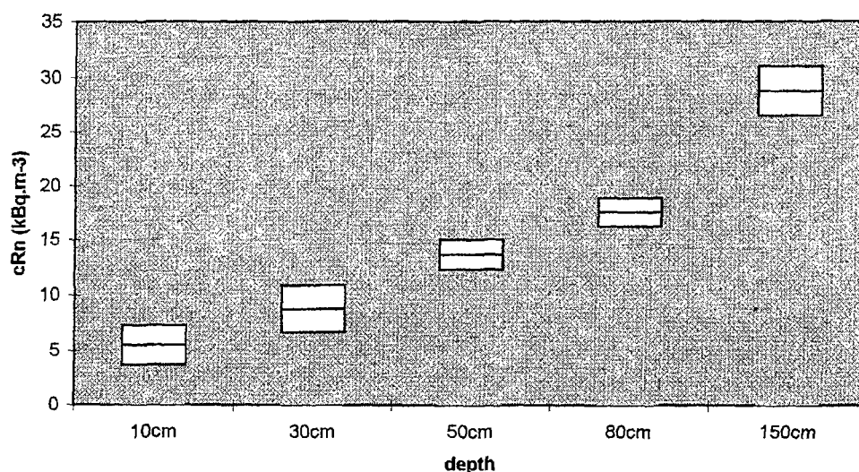
Fig. 1: Changes of soil-gas radon concentration (cRn) with depth (arithmetic mean \pm standard deviation), Březiněves area
