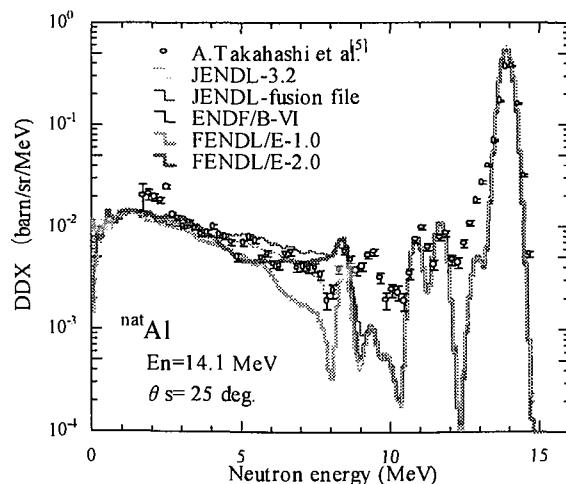
Fig.6 Evaluated neutron emission DDX of nat Al at 25 deg compared with the experimental data.
