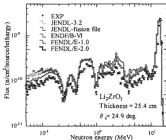
Fig.10 Neutron flux for \text{Li}_2\text{ZrO}_3 of 25.4 \text{ cm}^t at 24.9 \text{ deg} .
