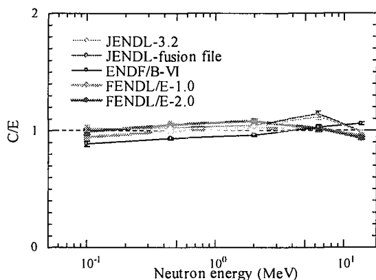
Fig.8 C/E for \text{Li}_2\text{TiO}_3 of 25.4 \text{ cm}^t at 24.9 \text{ deg} .
