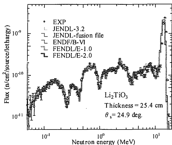
Fig.7 Neutron flux for \text{Li}_2\text{TiO}_3 of 25.4 \text{ cm}^t at 24.9 \text{ deg} .
