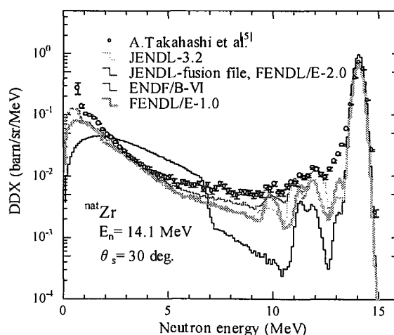
Fig.12 Evaluated neutron emission DDX of ^{nat}\text{Zr} at 30 \text{ deg} compared with the experimental data.
