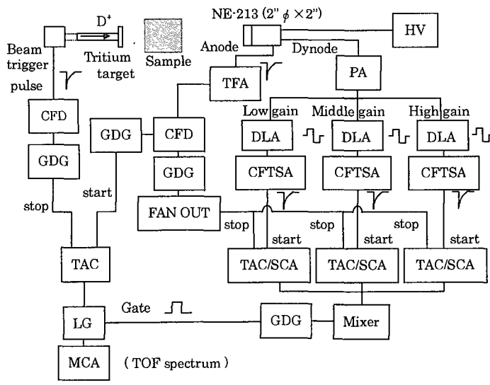
Fig.2 Block diagram of the measuring system
