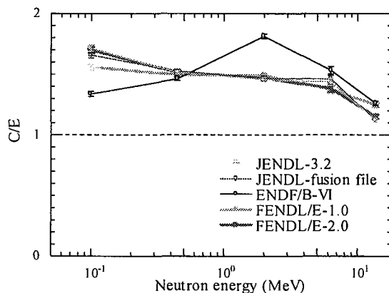
Fig.11 C/E for \text{Li}_2\text{ZrO}_3 of 25.4 \text{ cm}^t at 24.9 \text{ deg} .
