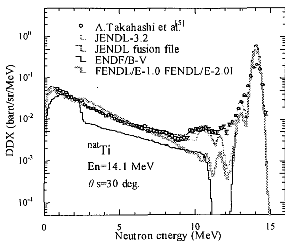
Fig.9 Evaluated neutron emission DDX of ^{nat}\text{Ti} at 30 \text{ deg} compared with the experimental data.
